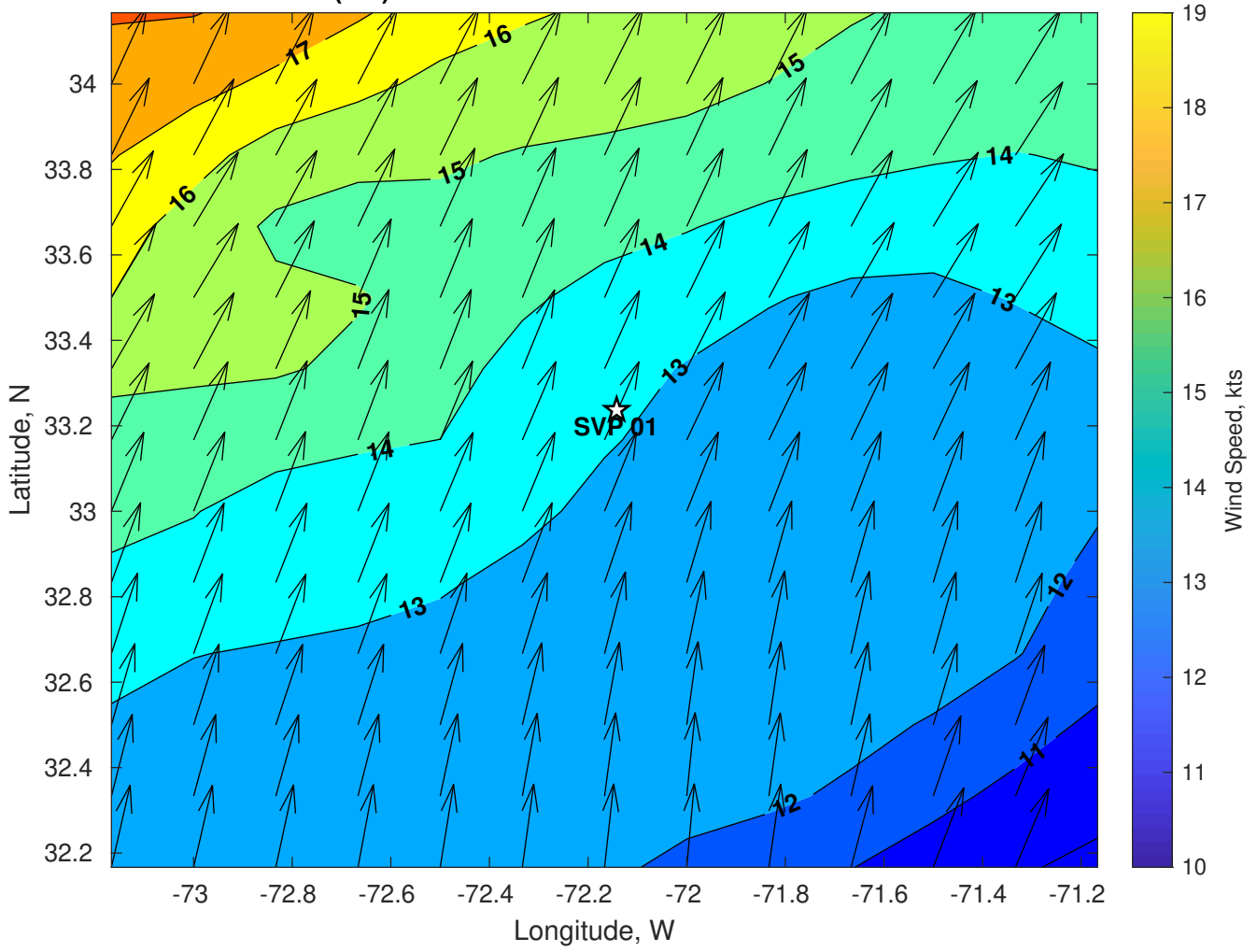
Winds (kts) for SVP 01 at 24-Jul-2024 06:00:00
