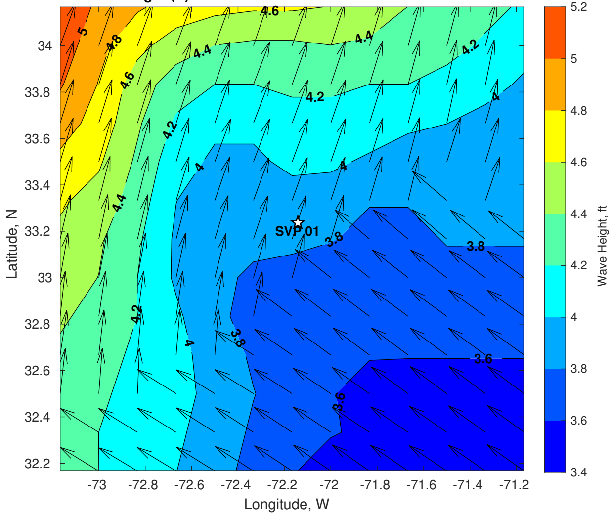
Wave Height (ft) for SVP 01 at 24-Jul-2024 06:00:00
