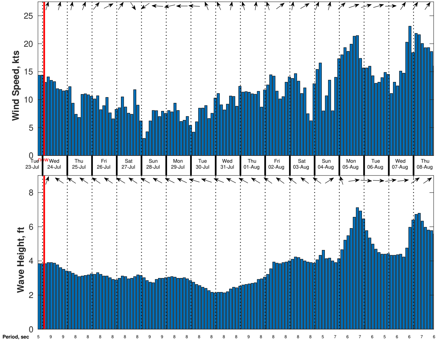
Wind & Wave Forecast for SVP 01 from 23-Jul-2024 19:00:00 to 08-Aug-2024 19:00:00
