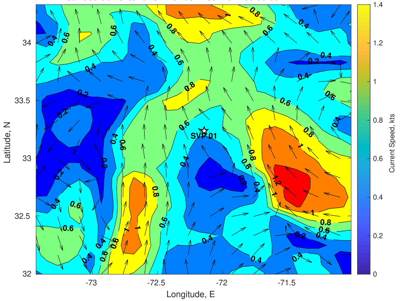
Surface Currents for SVP 01 at 24-Jul-2024 00:00:00
