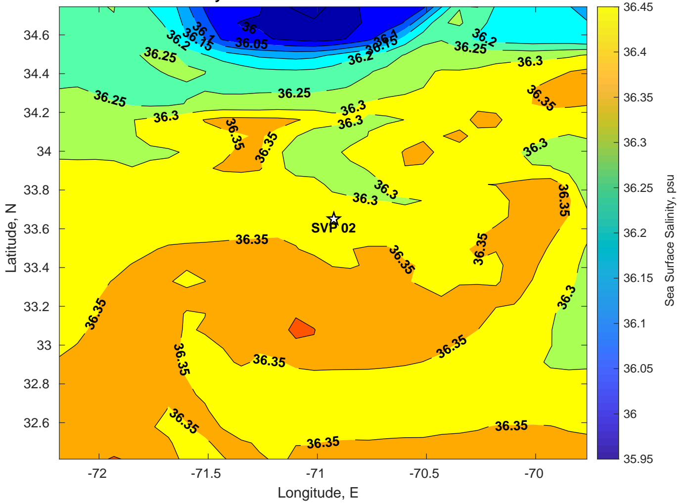
Surface Salinity for SVP 02 at 24-Jul-2024 00:00:00
