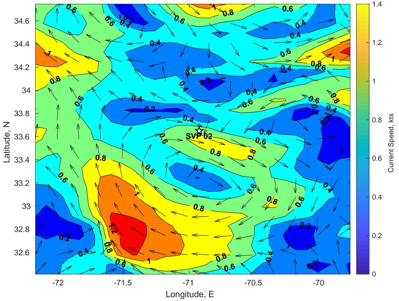
Surface Currents for SVP 02 at 24-Jul-2024 00:00:00
