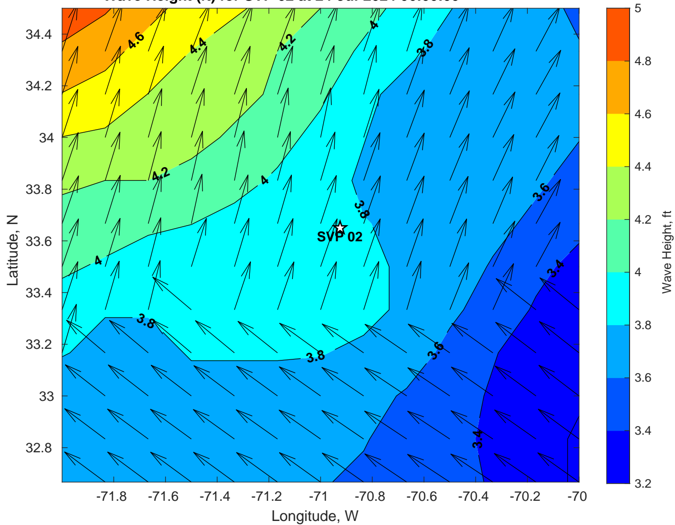
Wave Height (ft) for SVP 02 at 24-Jul-2024 06:00:00
