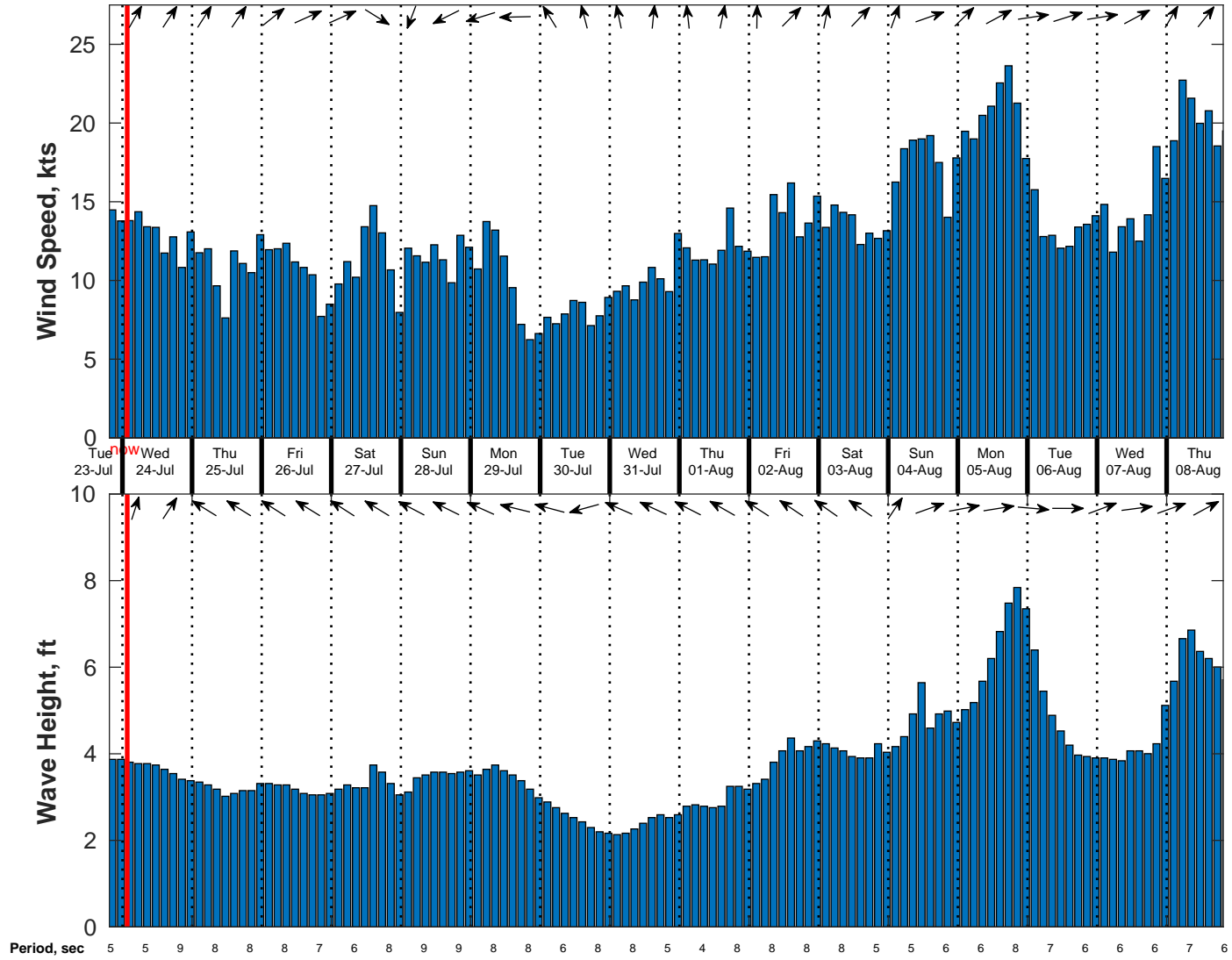
Wind & Wave Forecast for SVP 02 from 23-Jul-2024 19:00:00 to 08-Aug-2024 19:00:00
