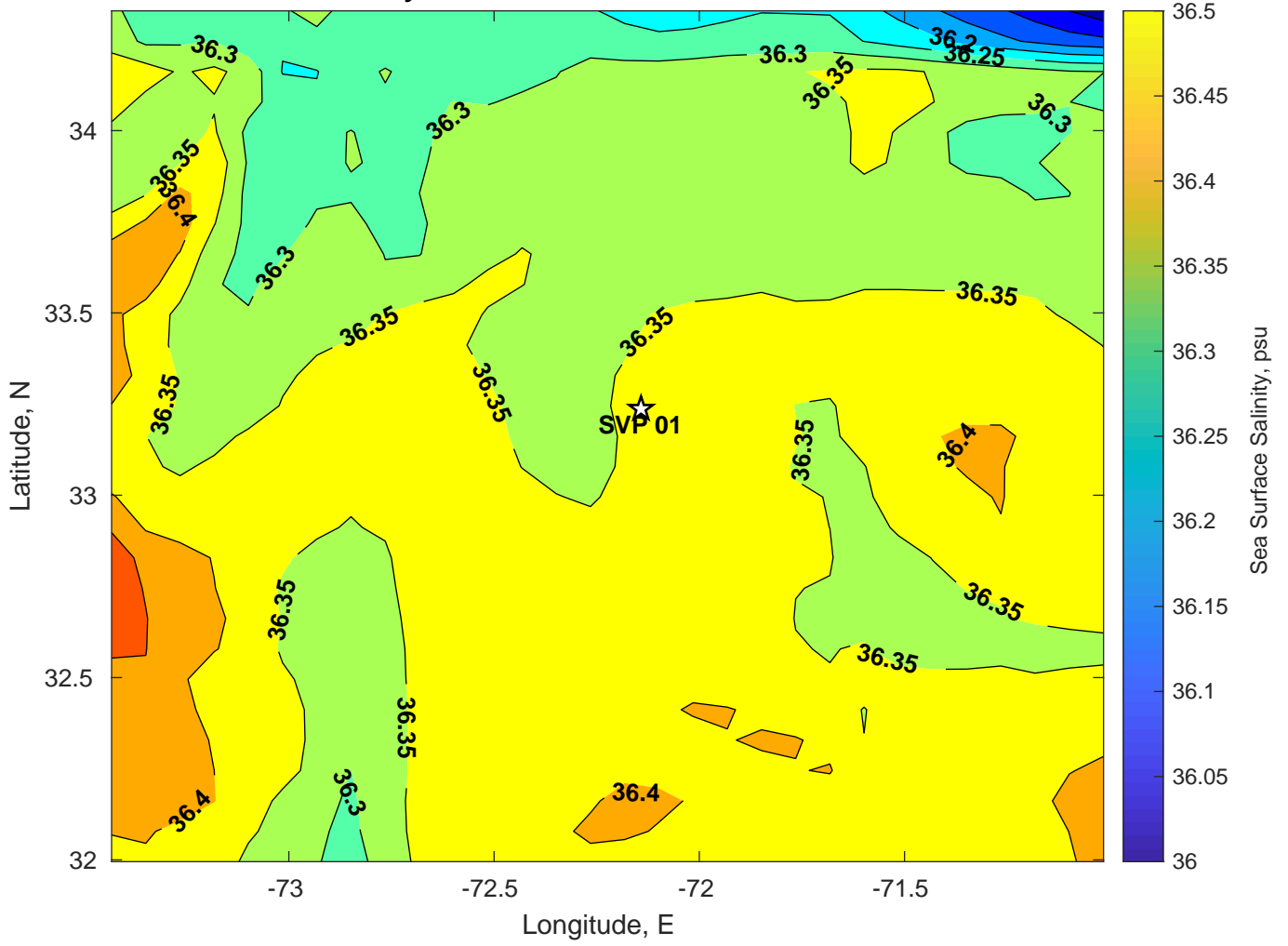
Surface Salinity for SVP 01 at 25-Jul-2024 00:00:00
