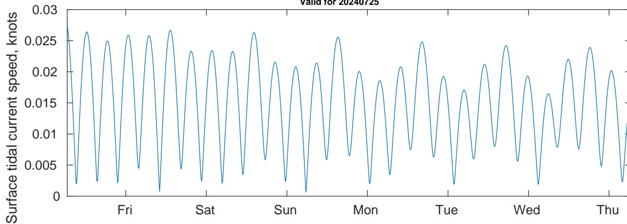
Tidal Currents and Heights for SVP 01 at 20240725
