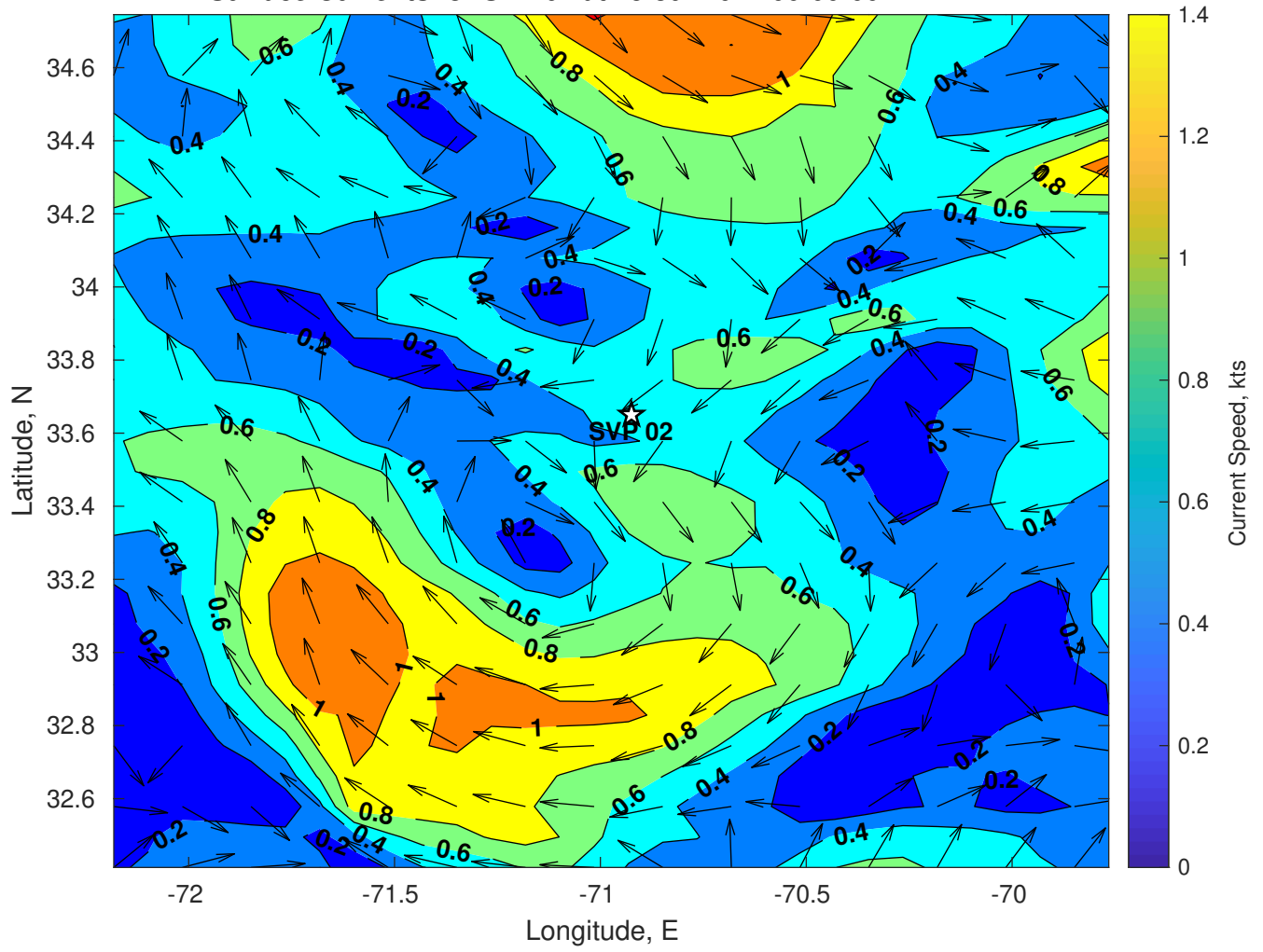
Surface Currents for SVP 02 at 25-Jul-2024 00:00:00
