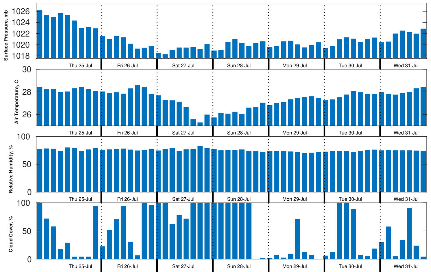
Met Forecast for SVP 02 from 25-Jul-2024 00:00:00 to 01-Aug-2024 00:00:00
