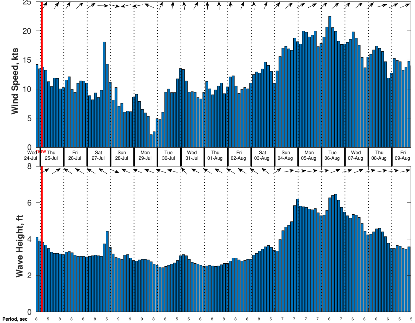
Wind & Wave Forecast for SVP 02 from 24-Jul-2024 19:00:00 to 09-Aug-2024 19:00:00
