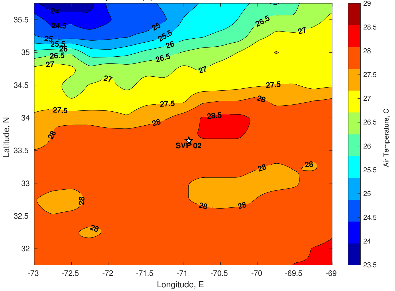
Air Temperature (C) for SVP 02 at 25-Jul-2024
