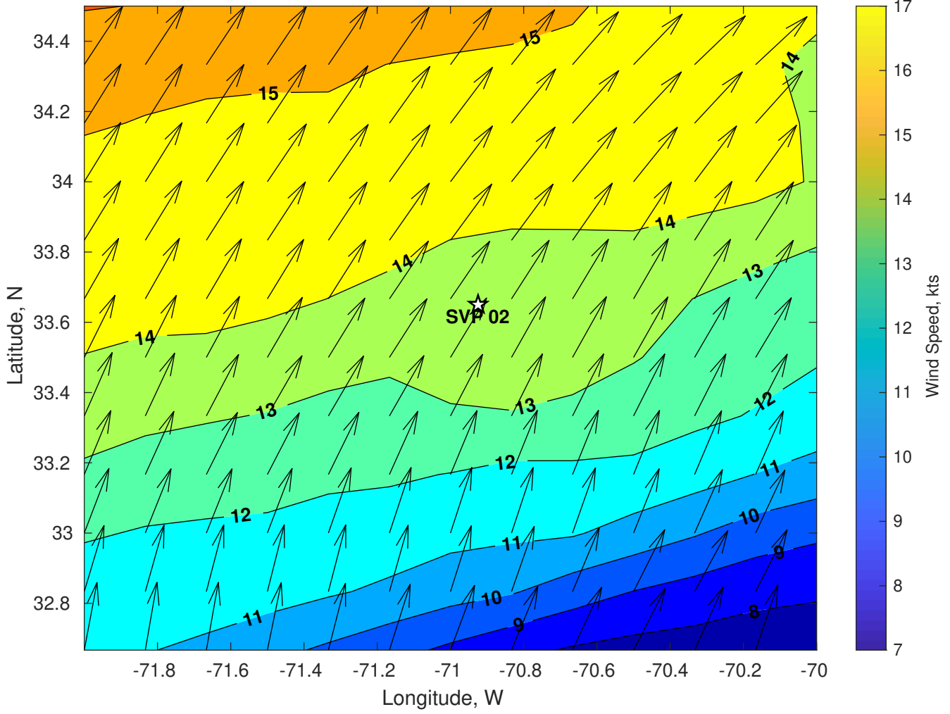
Winds (kts) for SVP 02 at 25-Jul-2024 06:00:00
