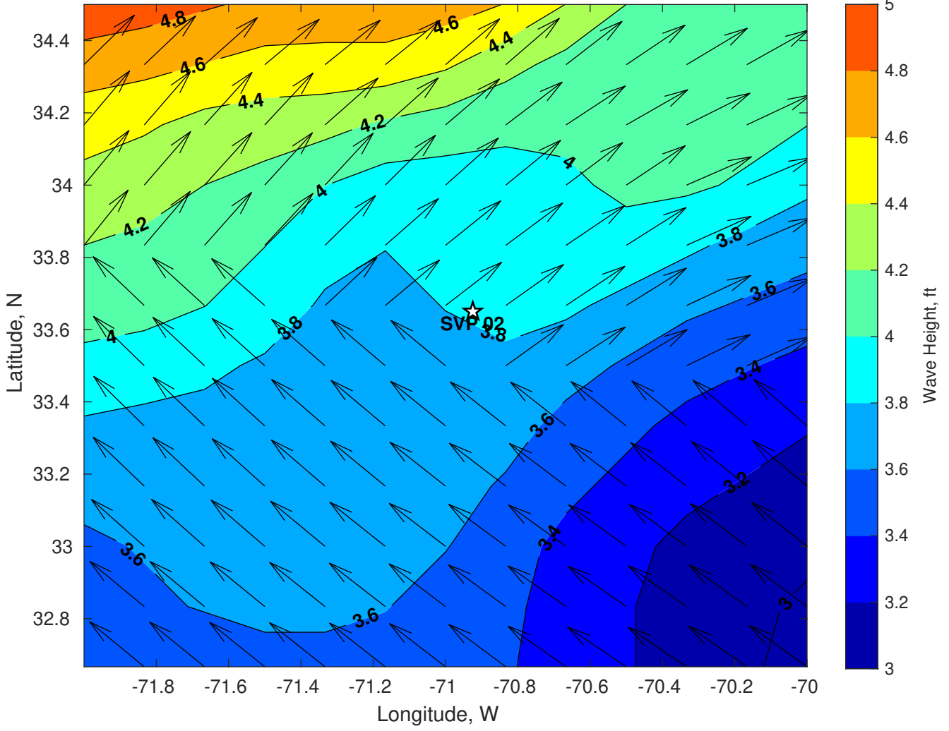
Wave Height (ft) for SVP 02 at 25-Jul-2024 06:00:00
