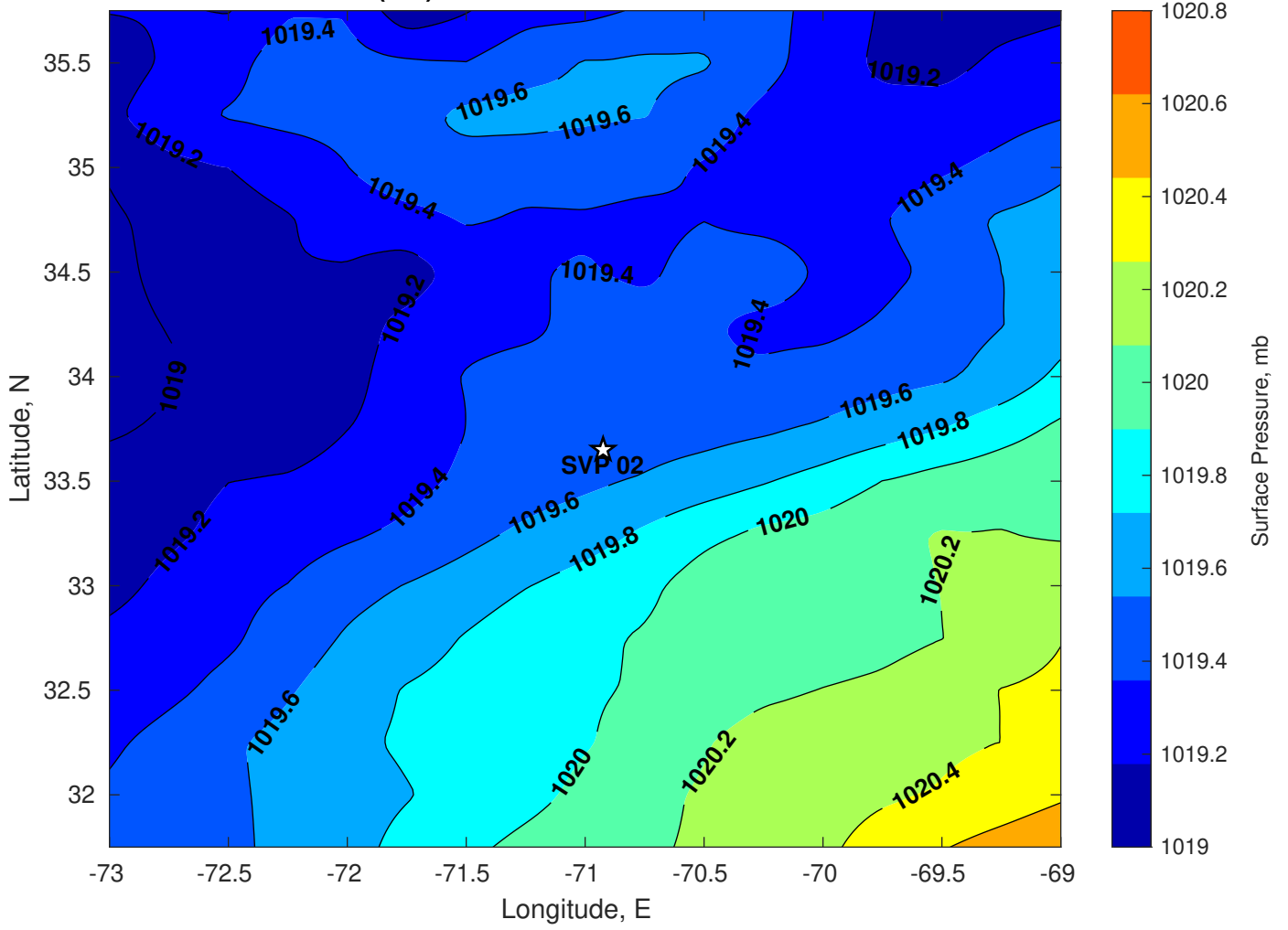
Surface Pressure (mb) for SVP 02 at 27-Jul-2024 00:00:00
