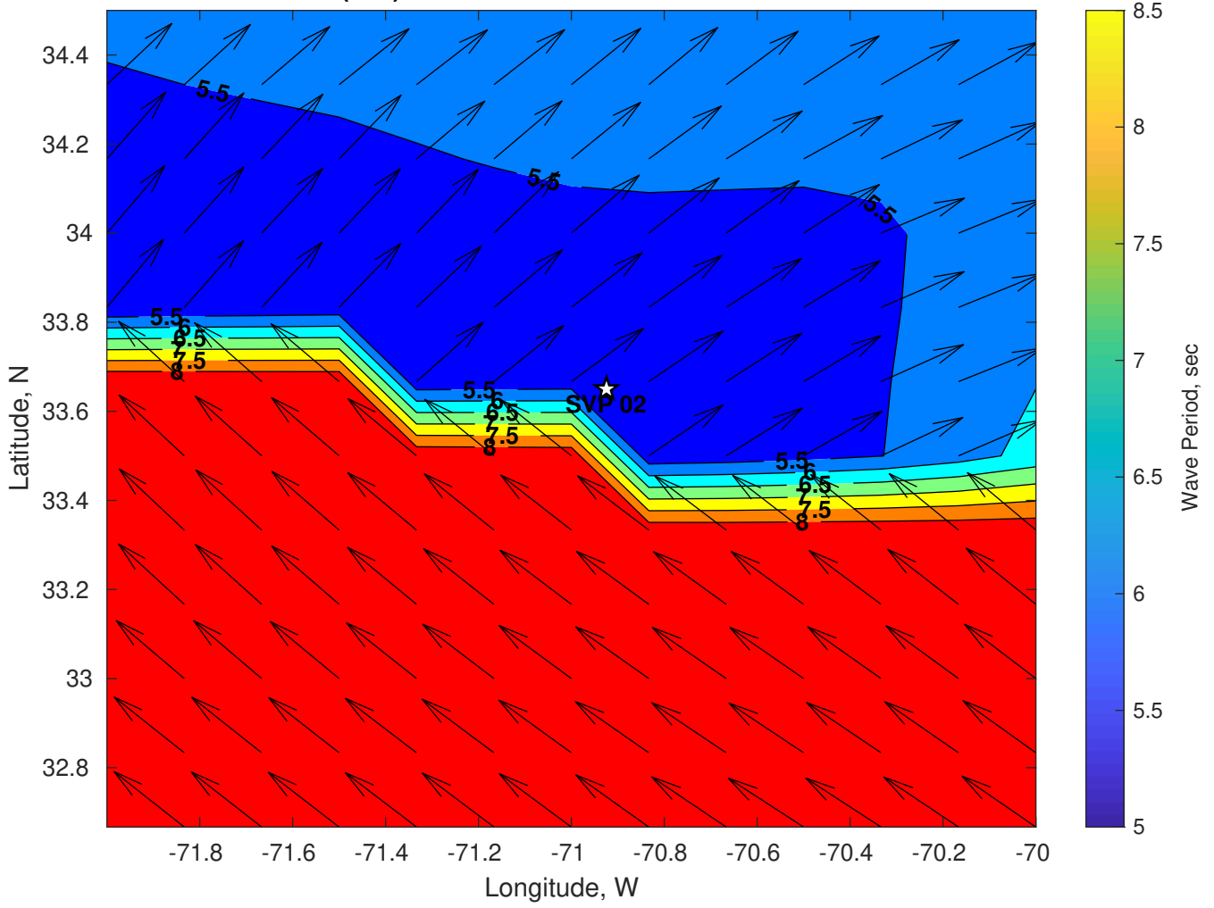
Wave Period (sec) for SVP 02 at 25-Jul-2024 06:00:00
