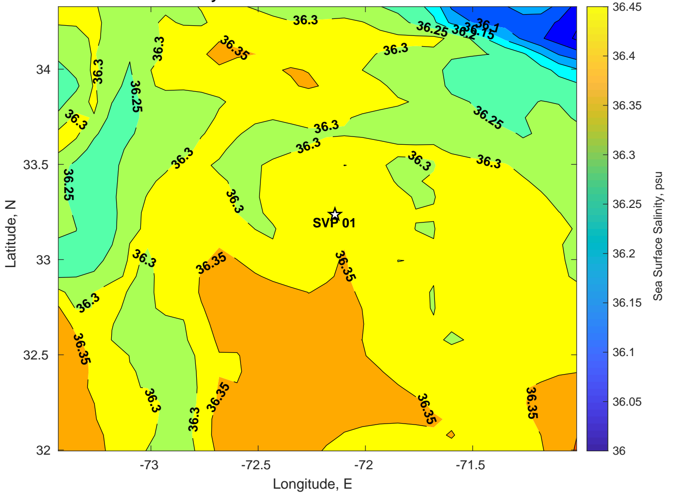
Surface Salinity for SVP 01 at 26-Jul-2024 00:00:00
