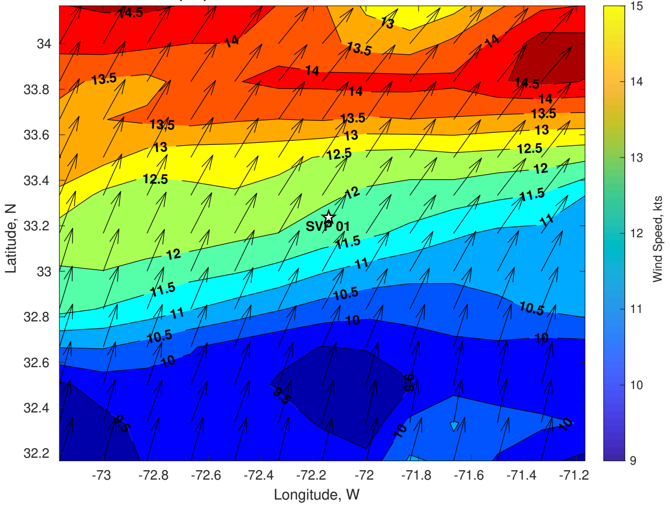
Winds (kts) for SVP 01 at 26-Jul-2024 06:00:00
