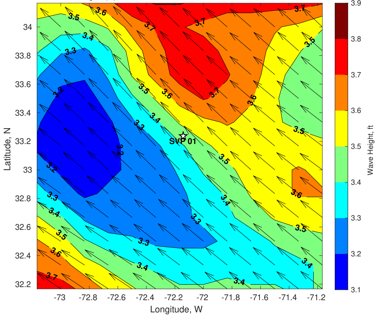
Wave Height (ft) for SVP 01 at 26-Jul-2024 06:00:00
