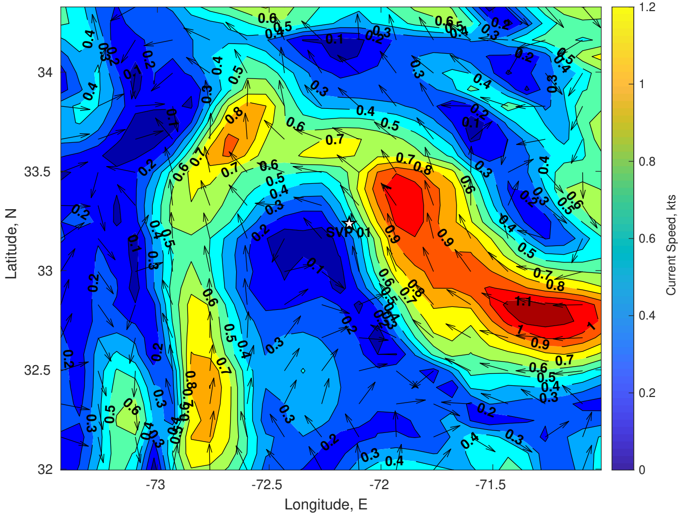
Surface Currents for SVP 01 at 26-Jul-2024 00:00:00
