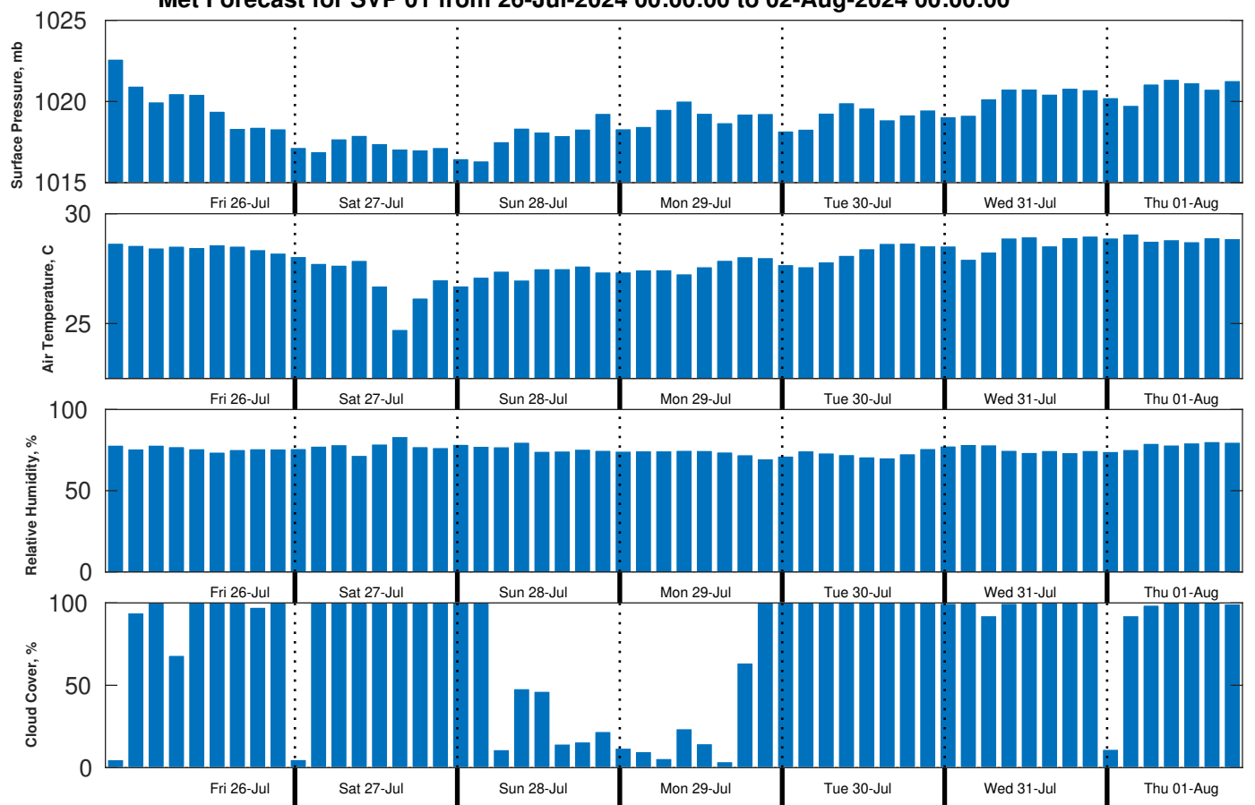
Met Forecast for SVP 01 from 26-Jul-2024 00:00:00 to 02-Aug-2024 00:00:00
