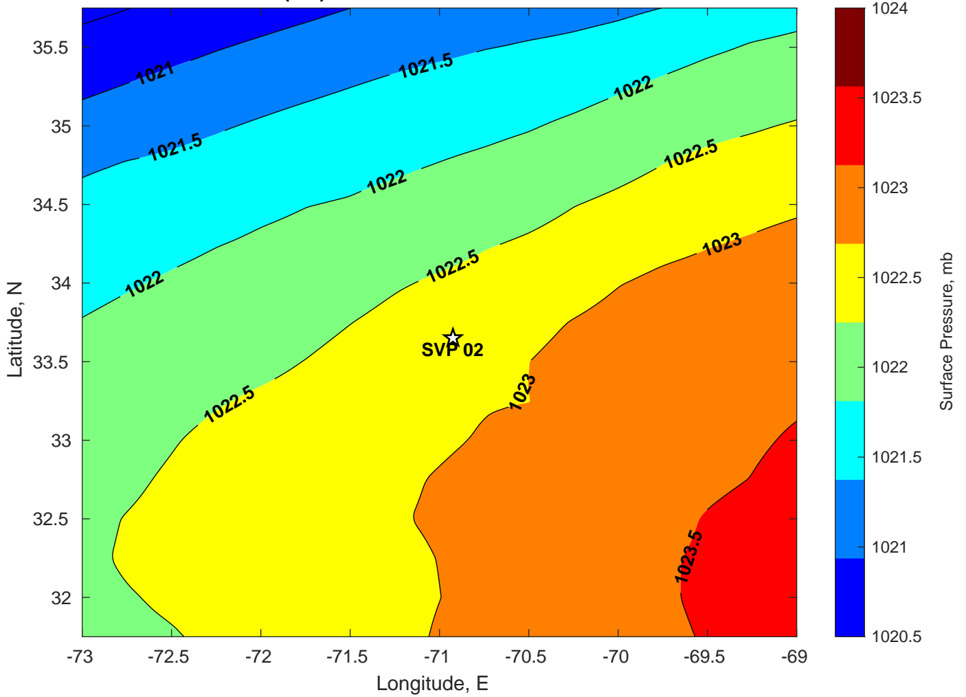
Surface Pressure (mb) for SVP 02 at 26-Jul-2024 00:00:00
