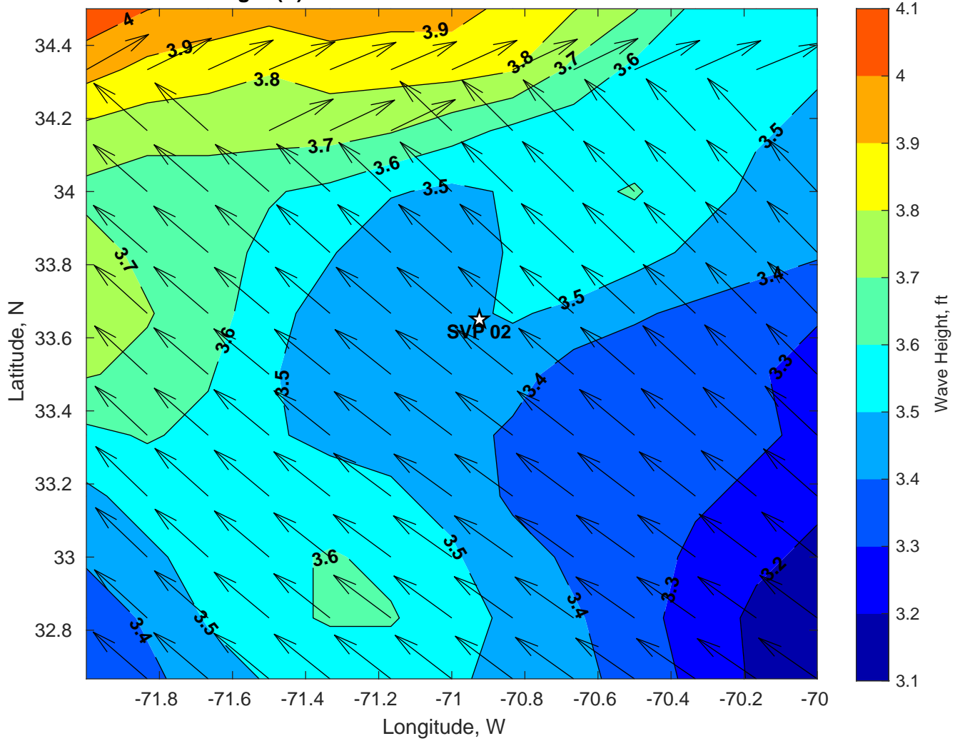
Wave Height (ft) for SVP 02 at 26-Jul-2024 06:00:00
