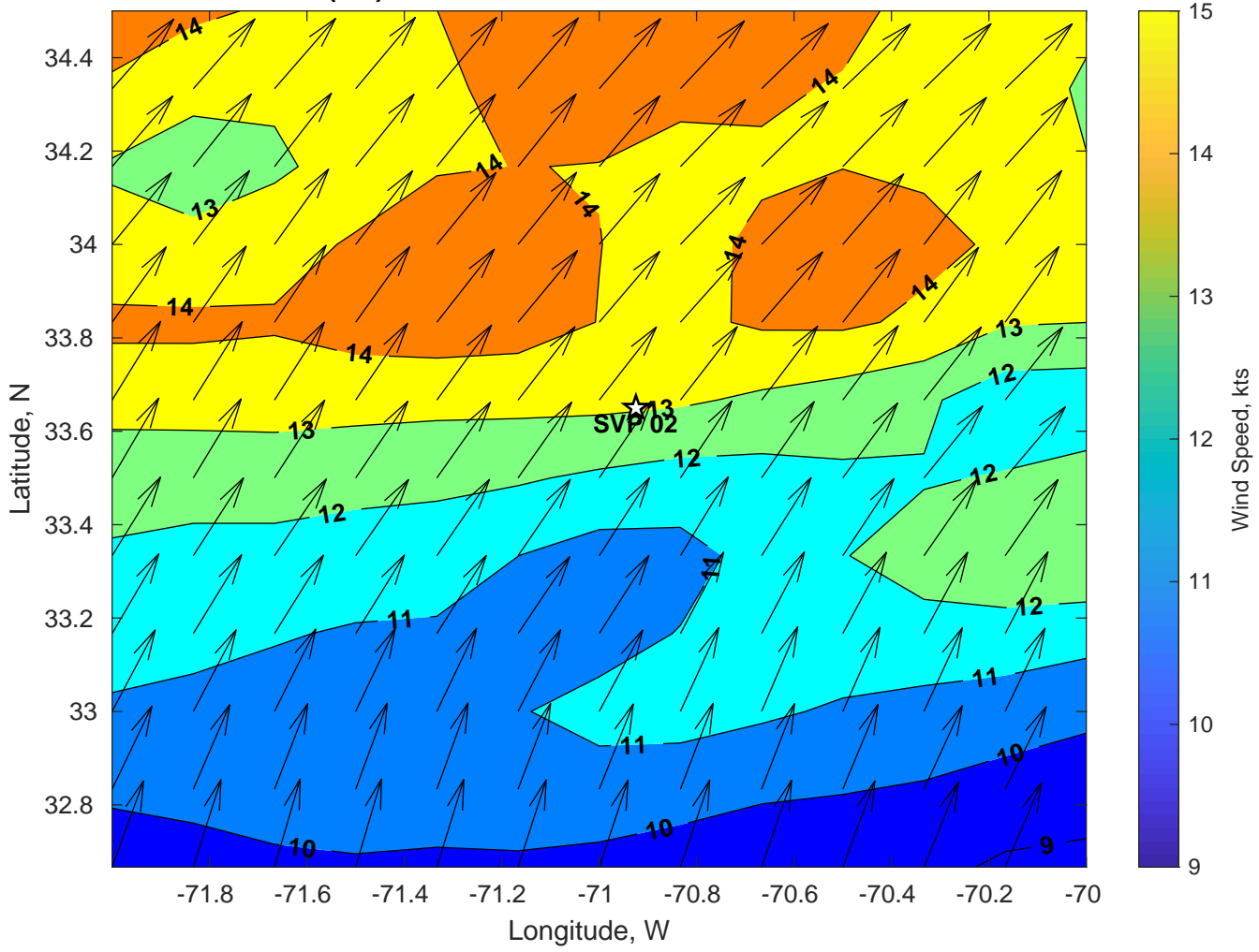
Winds (kts) for SVP 02 at 26-Jul-2024 06:00:00
