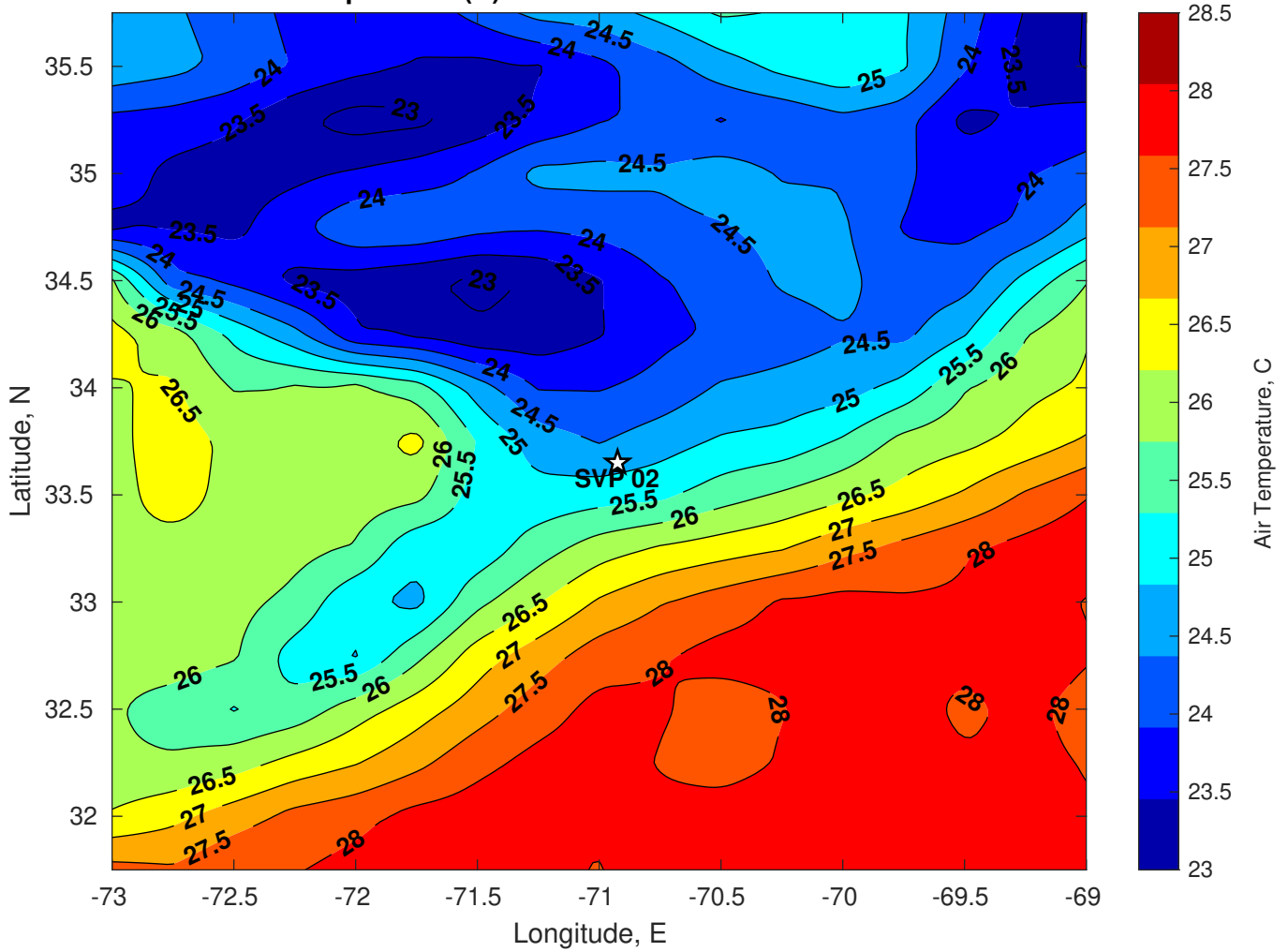
Air Temperature (C) for SVP 02 at 26-Jul-2024
