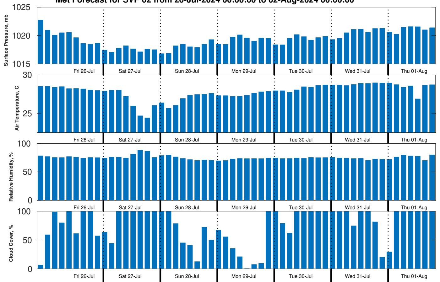
Met Forecast for SVP 02 from 26-Jul-2024 00:00:00 to 02-Aug-2024 00:00:00
