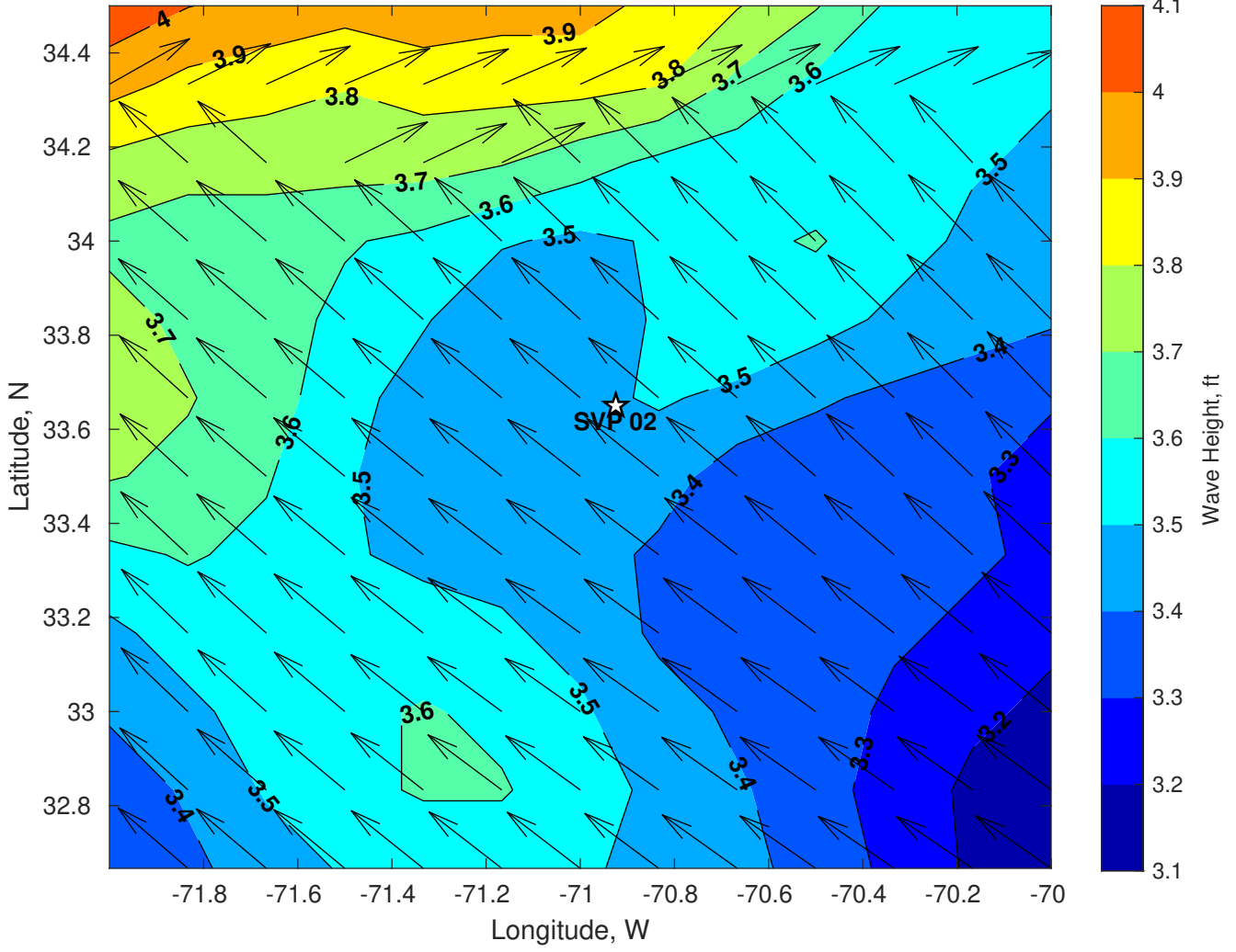
Wave Height (ft) for SVP 02 at 26-Jul-2024 06:00:00
