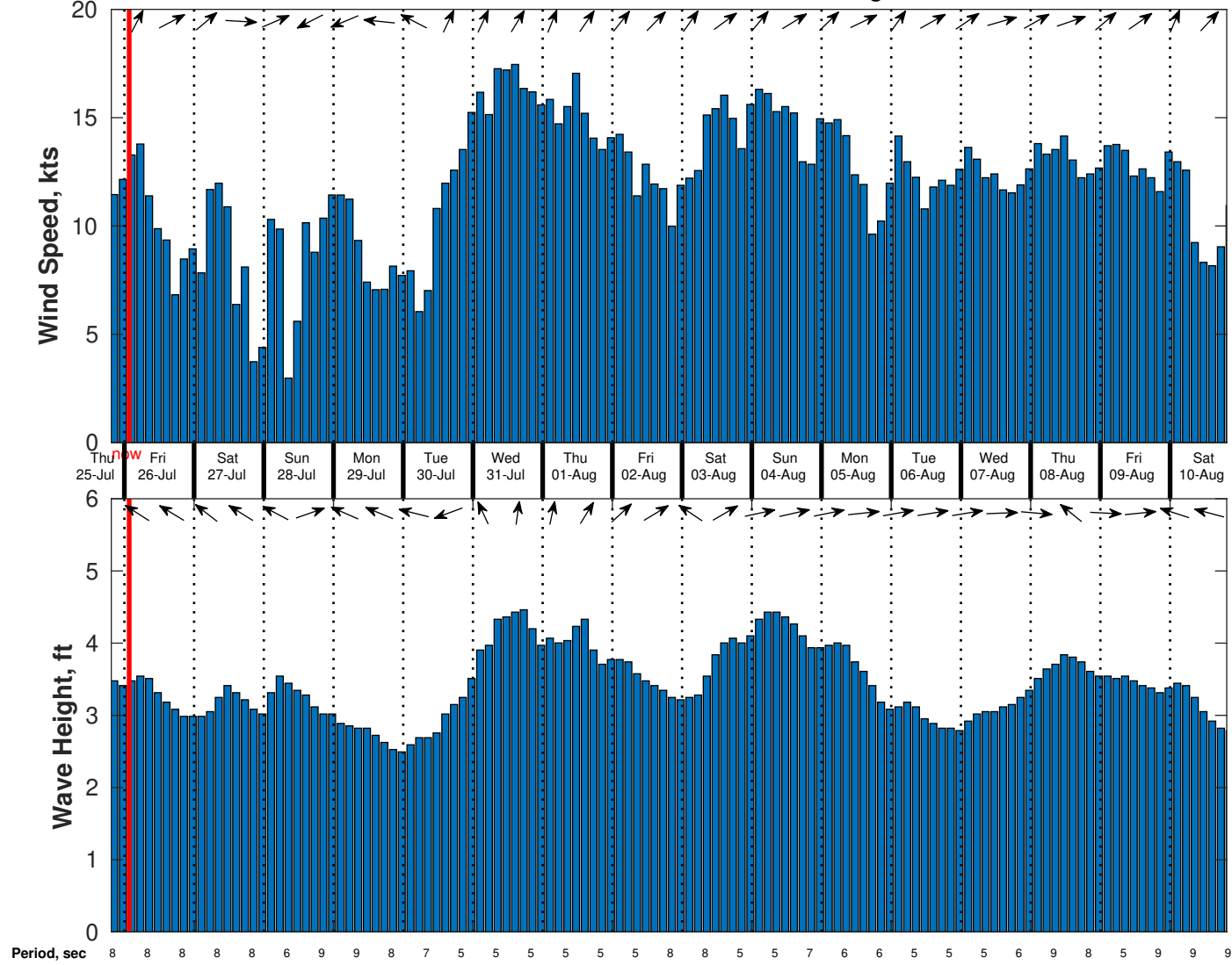
Wind & Wave Forecast for SVP 02 from 25-Jul-2024 19:00:00 to 10-Aug-2024 19:00:00
