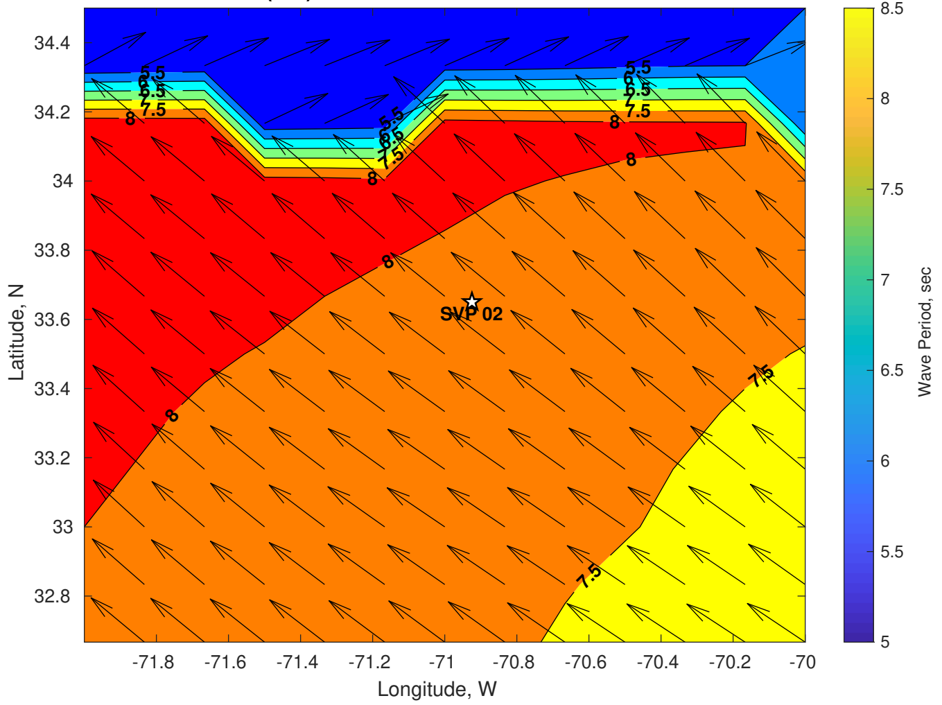
Wave Period (sec) for SVP 02 at 26-Jul-2024 06:00:00
