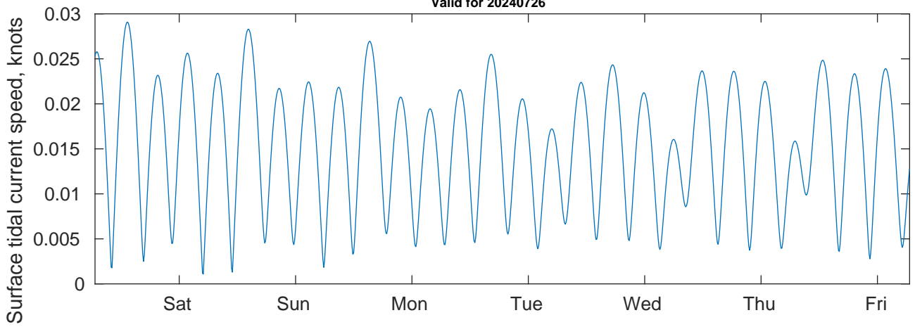
Tidal Currents and Heights for SVP 02 at 20240726
