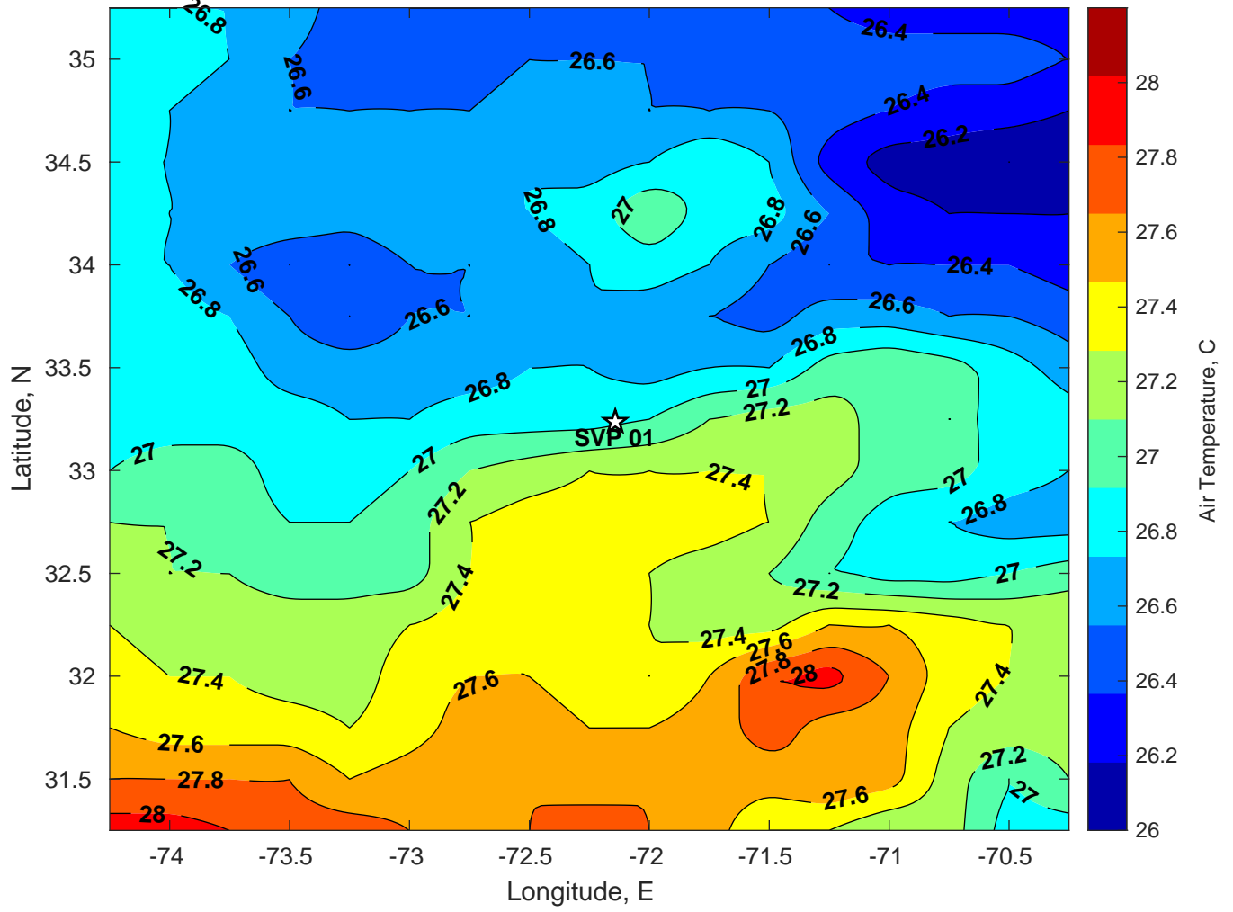
Air Temperature (C) for SVP 01 at 27-Jul-2024
