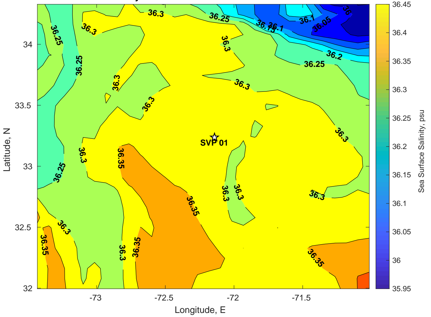
Surface Salinity for SVP 01 at 27-Jul-2024 00:00:00
