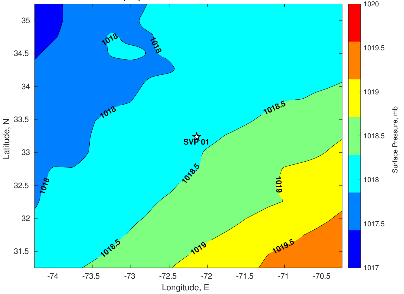
Surface Pressure (mb) for SVP 01 at 27-Jul-2024 00:00:00
