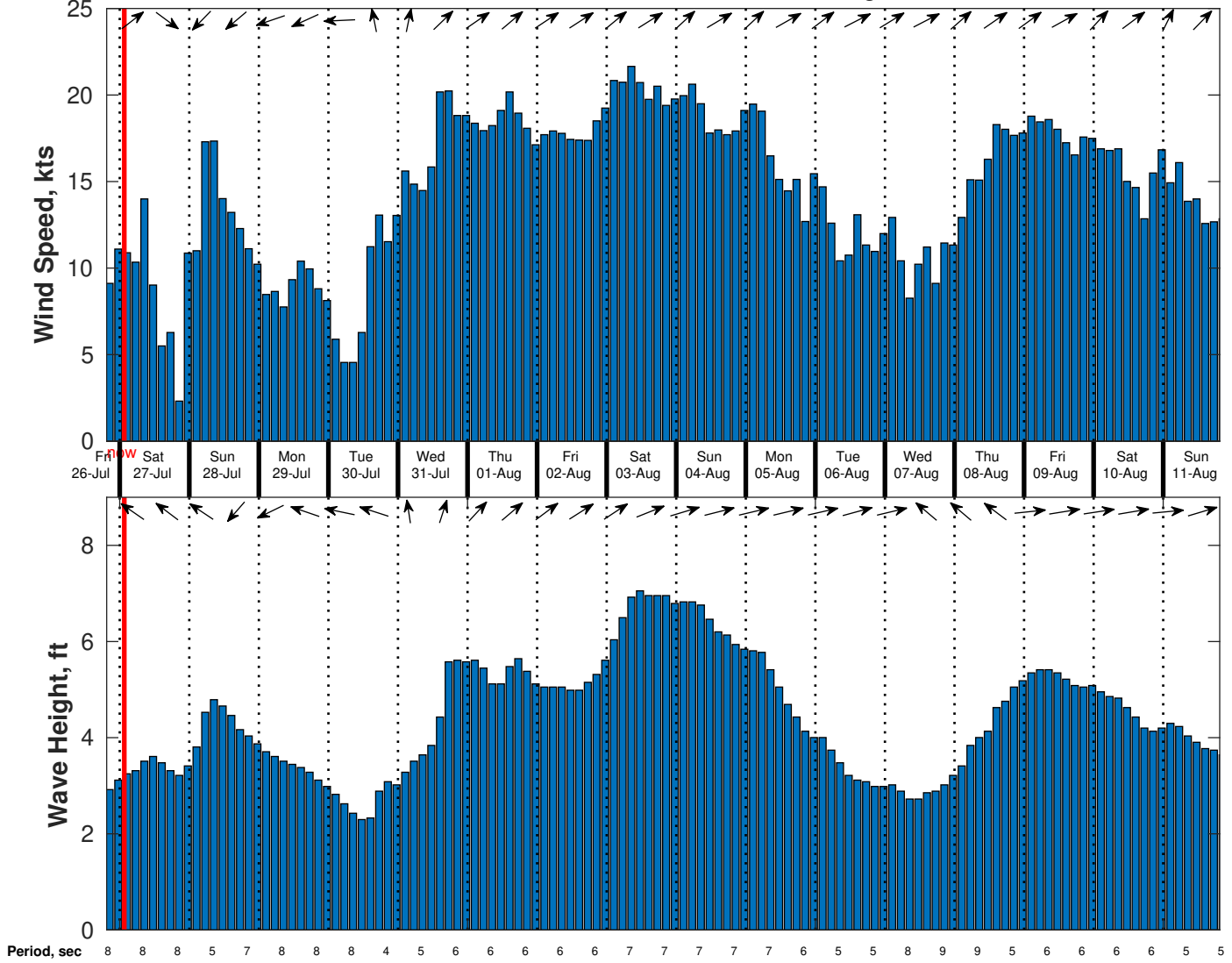
Wind & Wave Forecast for SVP 01 from 26-Jul-2024 19:00:00 to 11-Aug-2024 19:00:00
