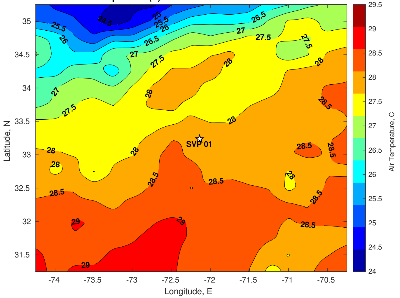
Air Temperature (C) for SVP 01 at 27-Jul-2024
