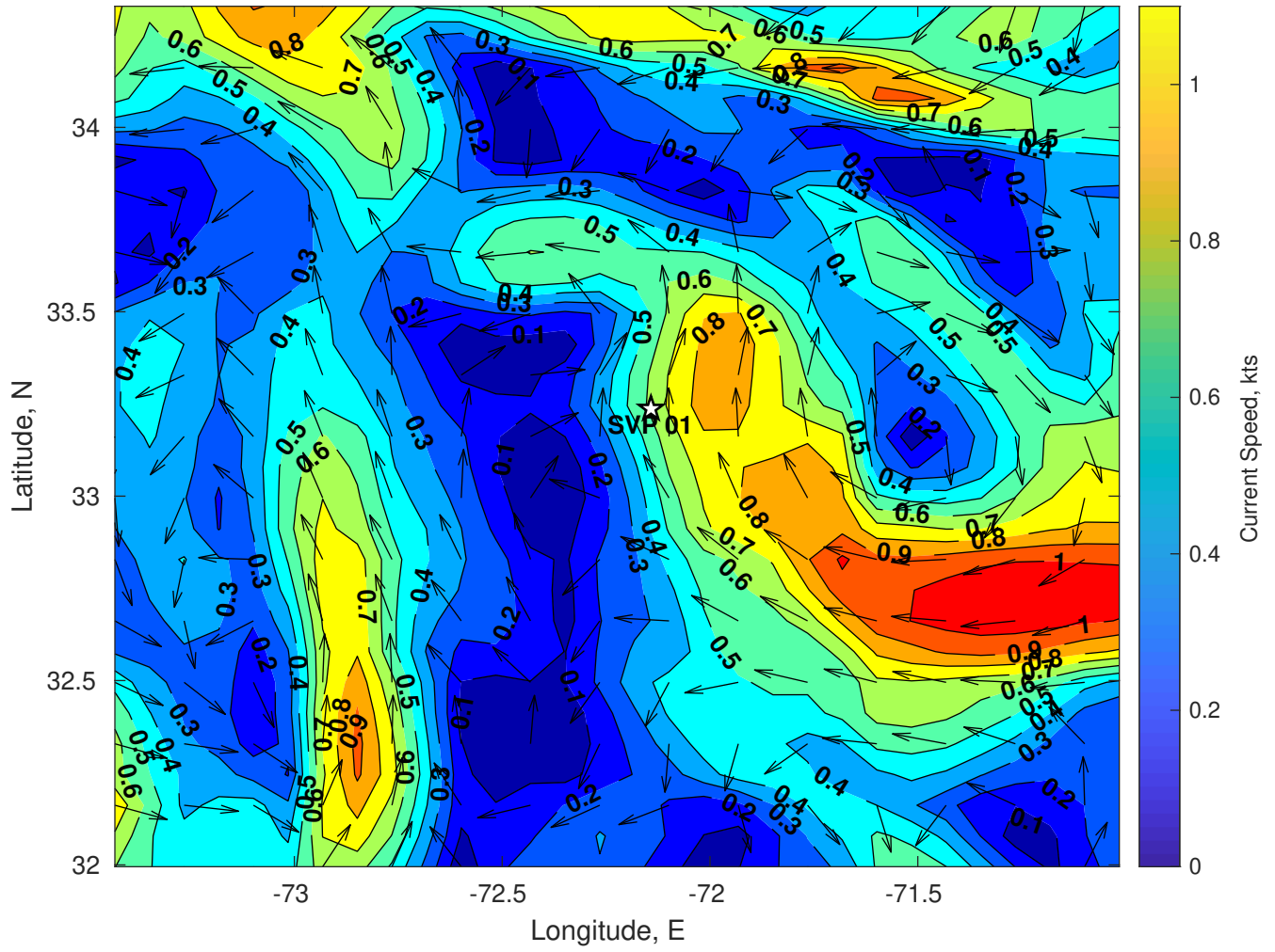
Surface Currents for SVP 01 at 27-Jul-2024 00:00:00
