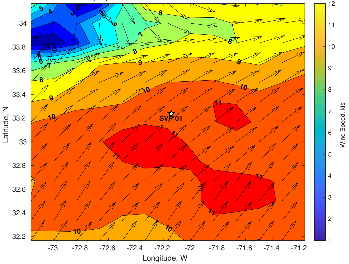
Winds (kts) for SVP 01 at 27-Jul-2024 06:00:00
