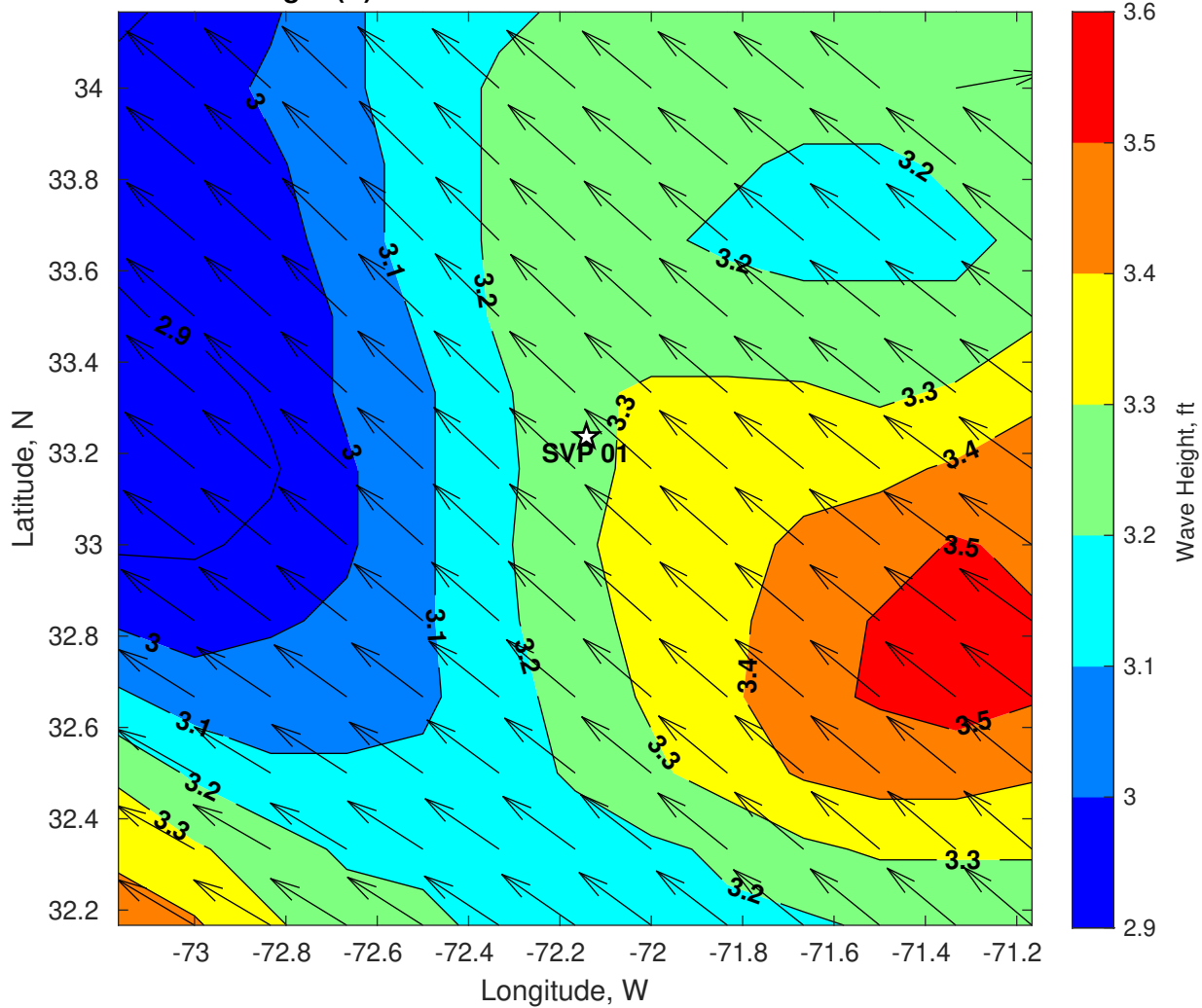
Wave Height (ft) for SVP 01 at 27-Jul-2024 06:00:00
