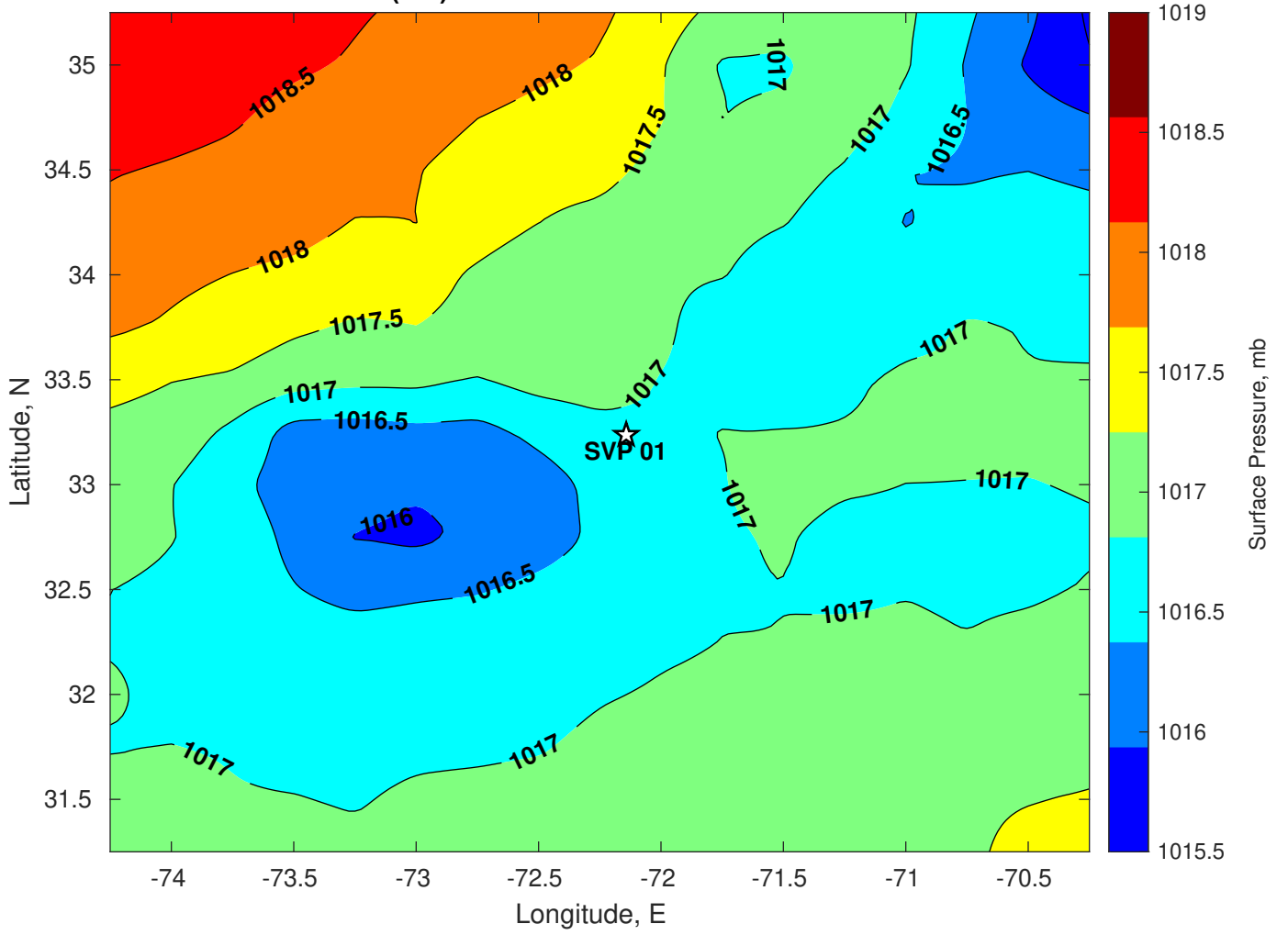
Surface Pressure (mb) for SVP 01 at 28-Jul-2024 00:00:00
