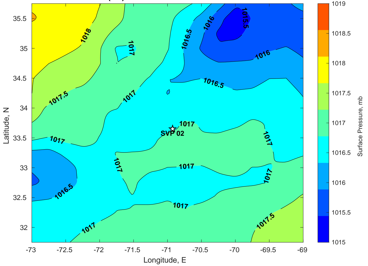
Surface Pressure (mb) for SVP 02 at 28-Jul-2024 00:00:00
