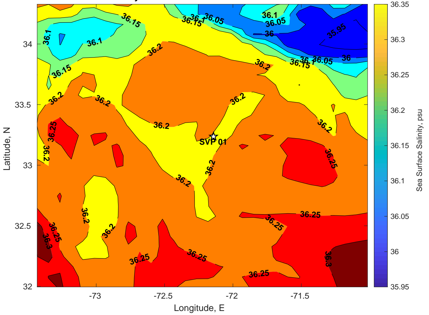
Surface Salinity for SVP 01 at 28-Jul-2024 00:00:00
