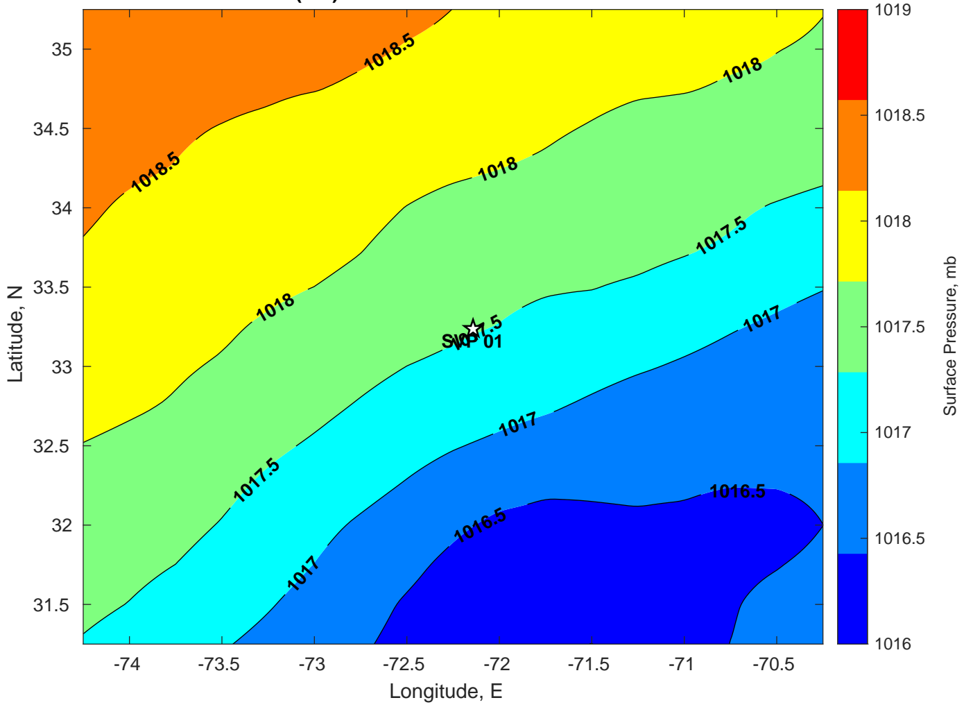
Surface Pressure (mb) for SVP 01 at 29-Jul-2024 00:00:00
