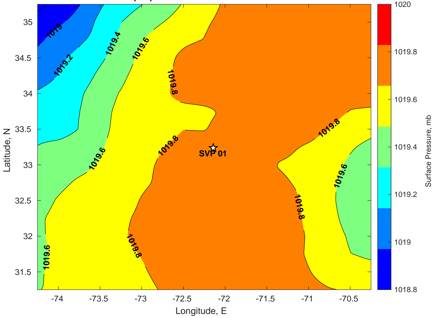
Surface Pressure (mb) for SVP 01 at 30-Jul-2024 00:00:00
