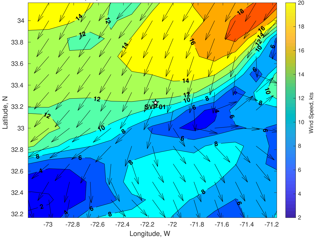
Winds (kts) for SVP 01 at 28-Jul-2024 06:00:00
