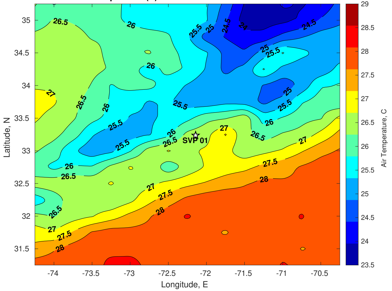
Air Temperature (C) for SVP 01 at 28-Jul-2024
