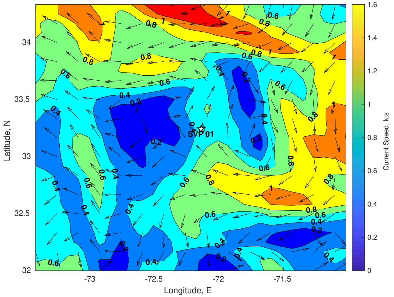
Surface Currents for SVP 01 at 28-Jul-2024 00:00:00
