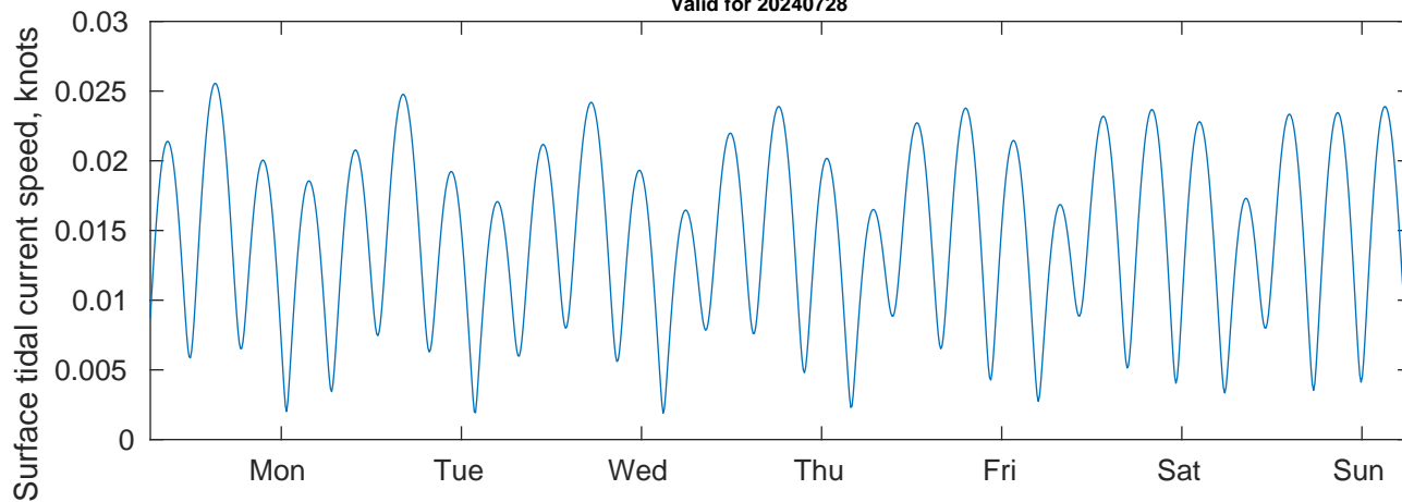
Tidal Currents and Heights for SVP 01 at 20240728
