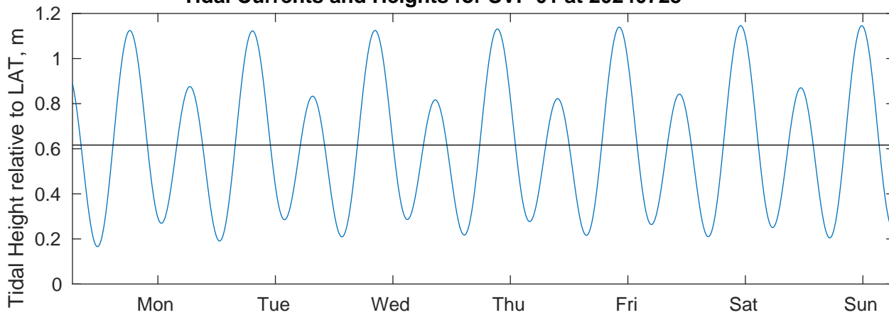
Tidal Currents and Heights for SVP 01 at 20240728
