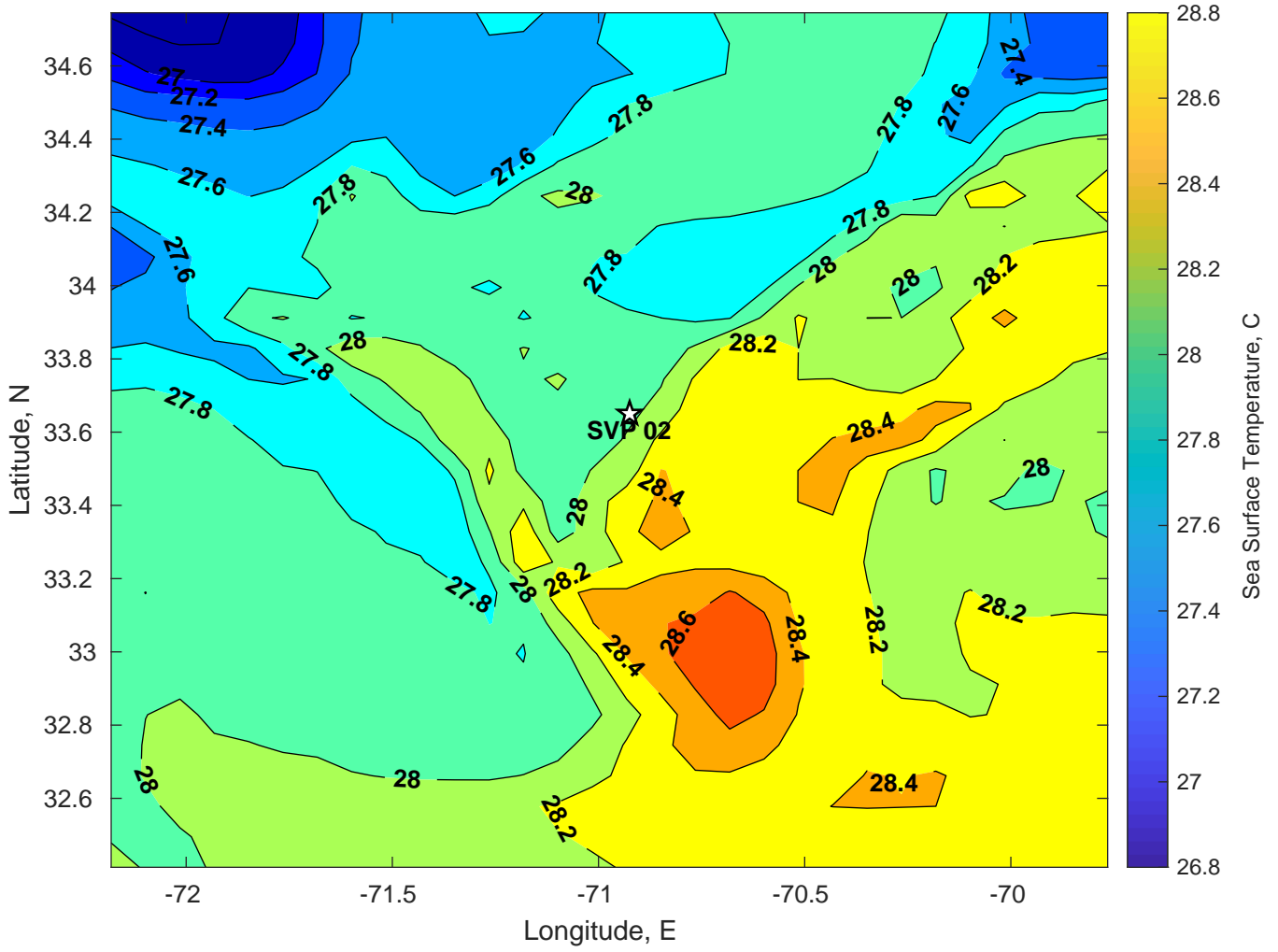
SST for SVP 02 at 28-Jul-2024 00:00:00
