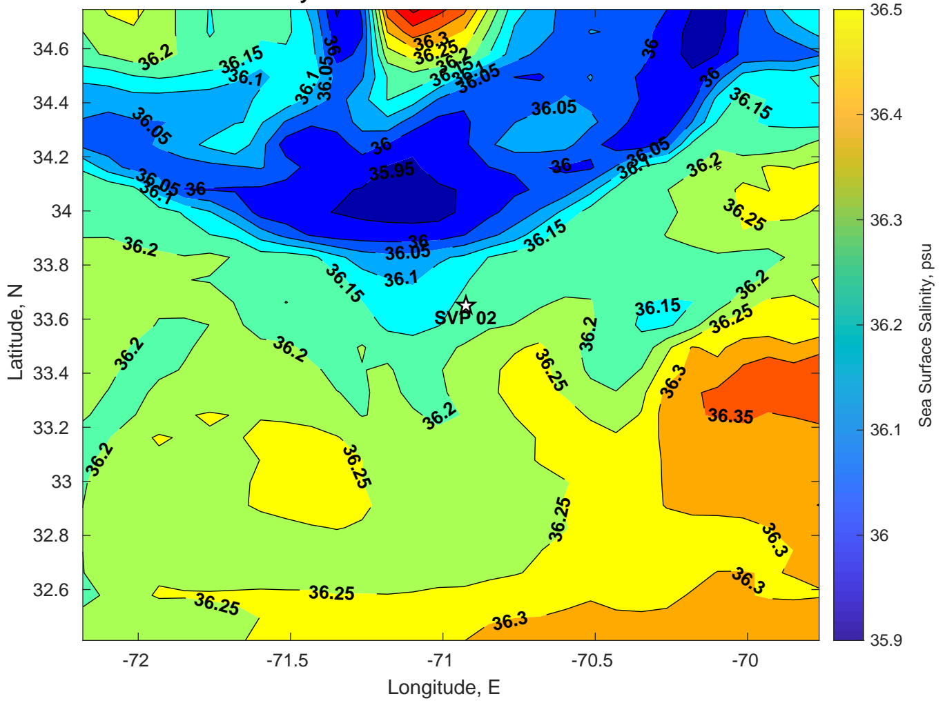
Surface Salinity for SVP 02 at 28-Jul-2024 00:00:00
