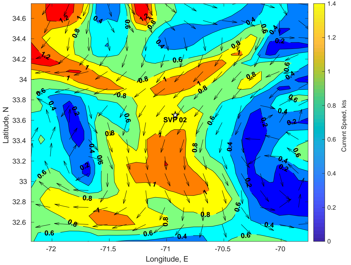
Surface Currents for SVP 02 at 28-Jul-2024 00:00:00
