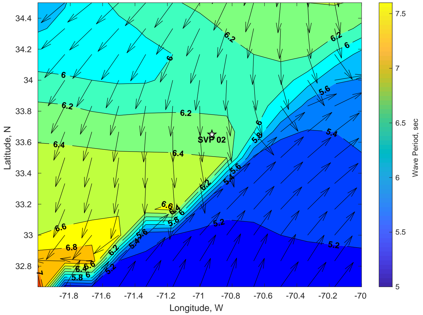
Wave Period (sec) for SVP 02 at 28-Jul-2024 06:00:00
