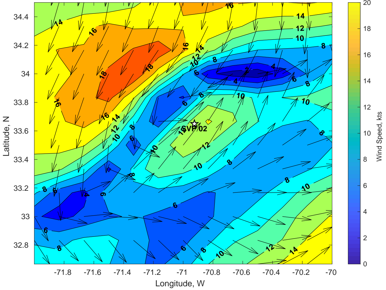
Winds (kts) for SVP 02 at 28-Jul-2024 06:00:00
