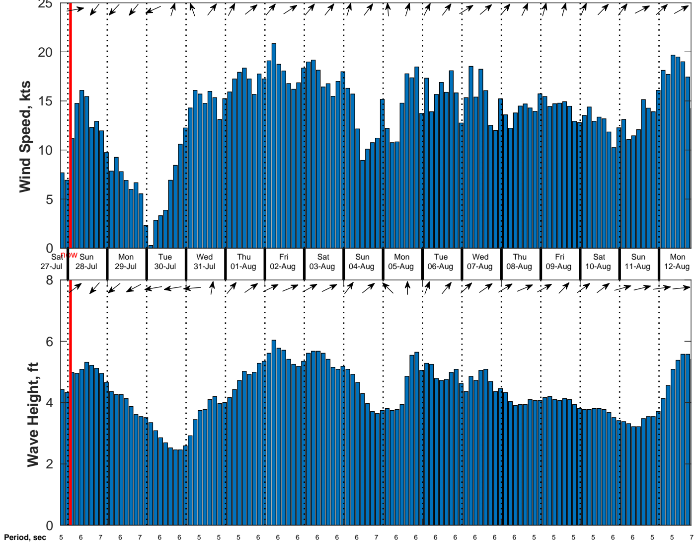
Wind & Wave Forecast for SVP 02 from 27-Jul-2024 19:00:00 to 12-Aug-2024 19:00:00
