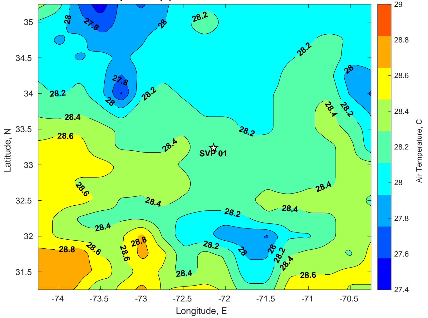
Air Temperature (C) for SVP 01 at 30-Jul-2024
