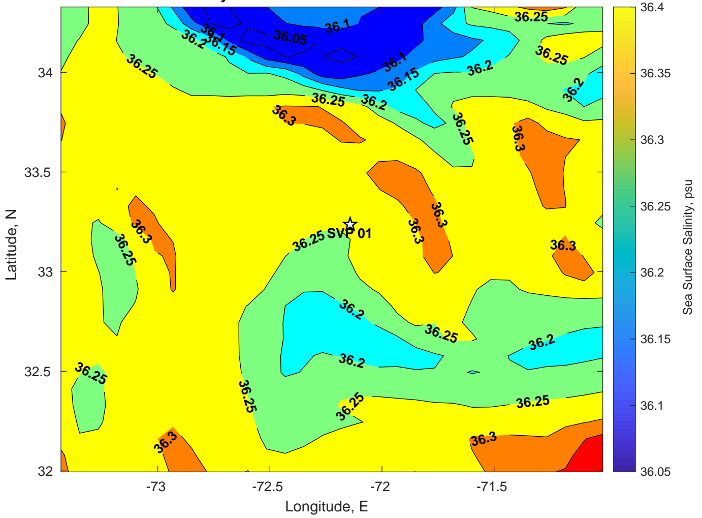
Surface Salinity for SVP 01 at 30-Jul-2024 00:00:00
