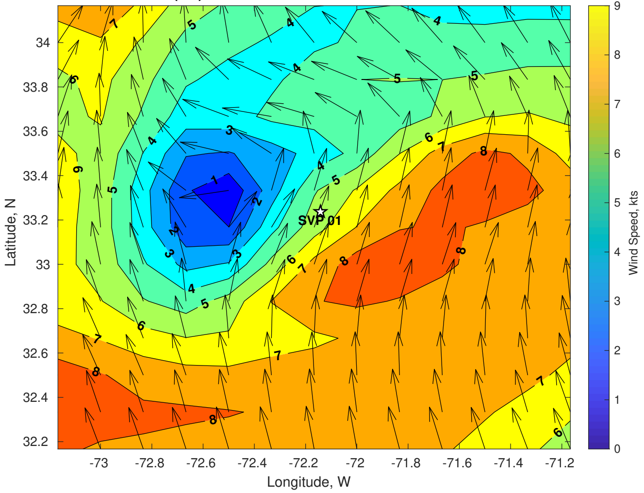
Winds (kts) for SVP 01 at 30-Jul-2024 06:00:00
