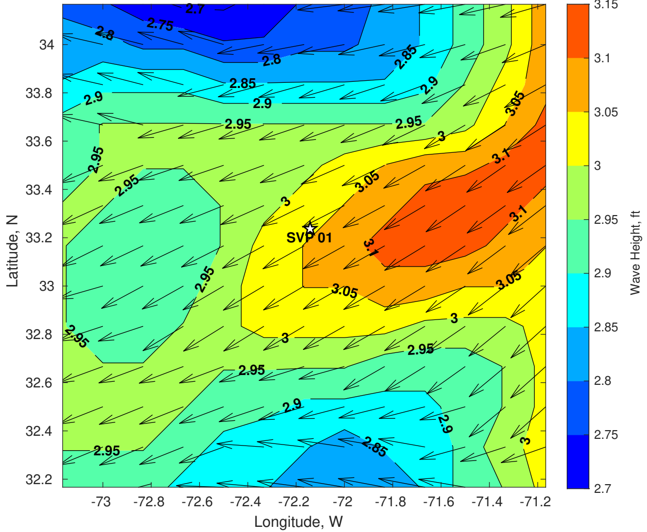
Wave Height (ft) for SVP 01 at 30-Jul-2024 06:00:00
