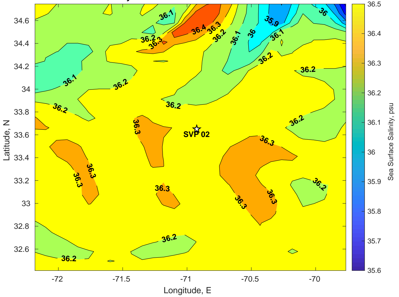
Surface Salinity for SVP 02 at 30-Jul-2024 00:00:00
