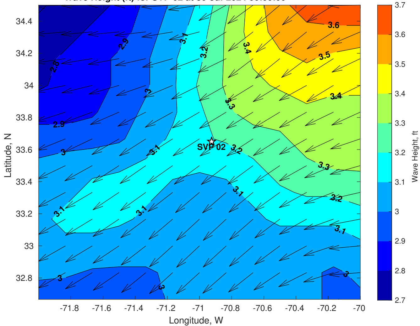
Wave Height (ft) for SVP 02 at 30-Jul-2024 06:00:00
