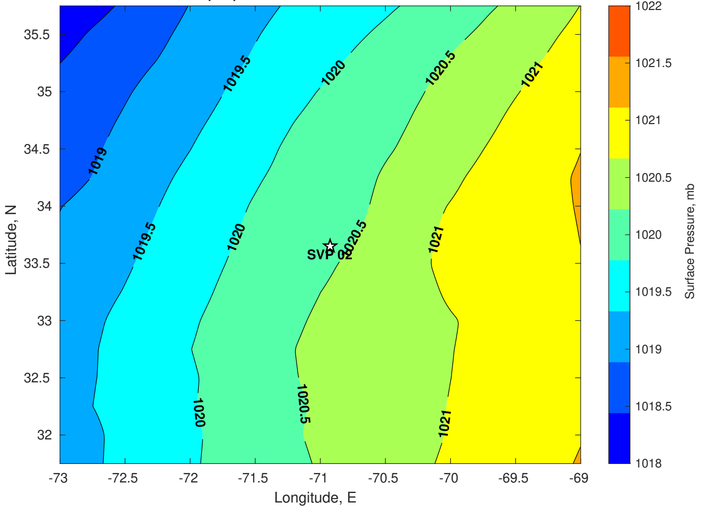
Surface Pressure (mb) for SVP 02 at 31-Jul-2024 00:00:00
