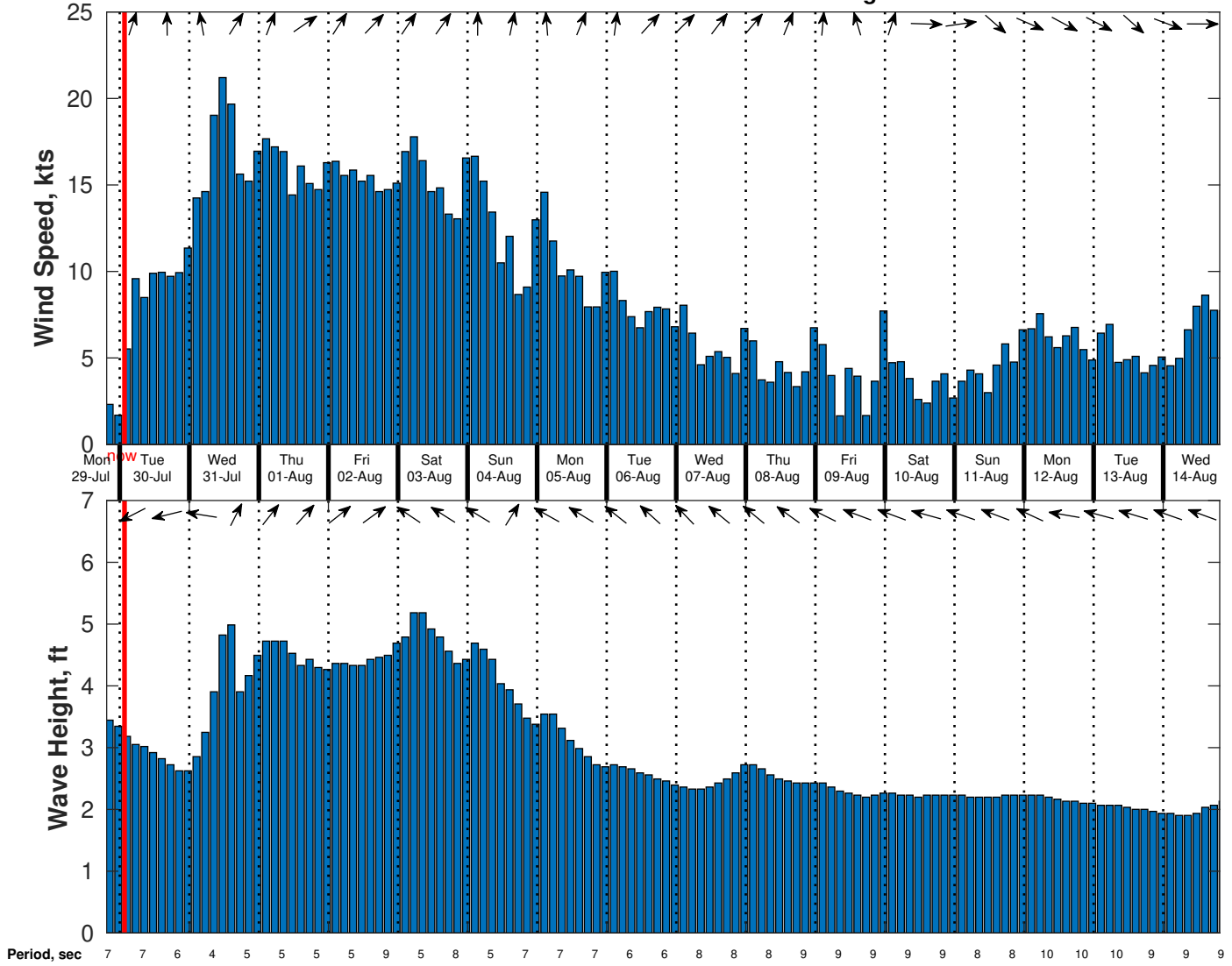
Wind & Wave Forecast for SVP 02 from 29-Jul-2024 19:00:00 to 14-Aug-2024 19:00:00
