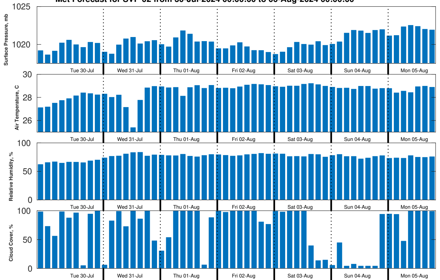
Met Forecast for SVP 02 from 30-Jul-2024 00:00:00 to 06-Aug-2024 00:00:00
