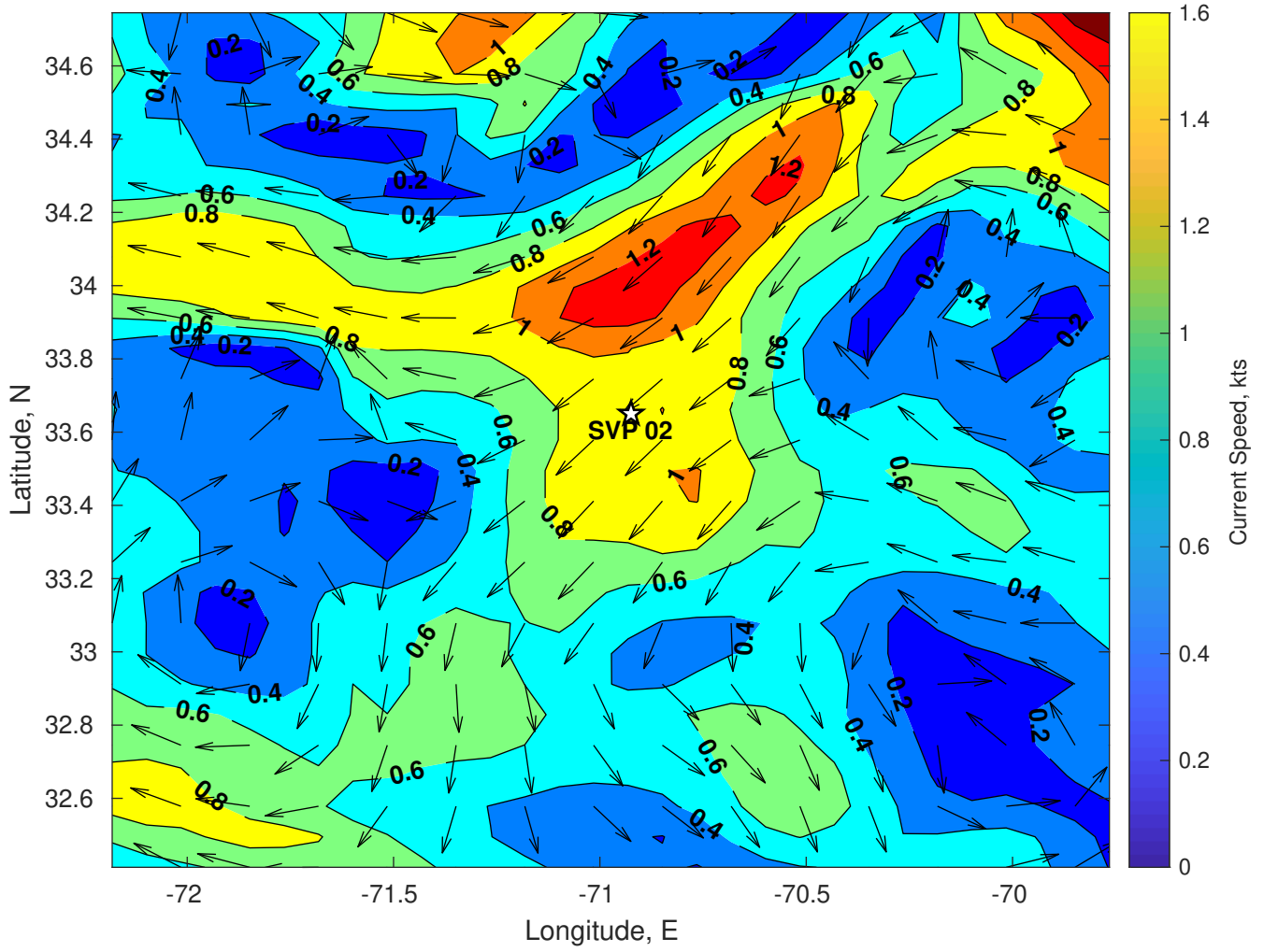
Surface Currents for SVP 02 at 30-Jul-2024 00:00:00
