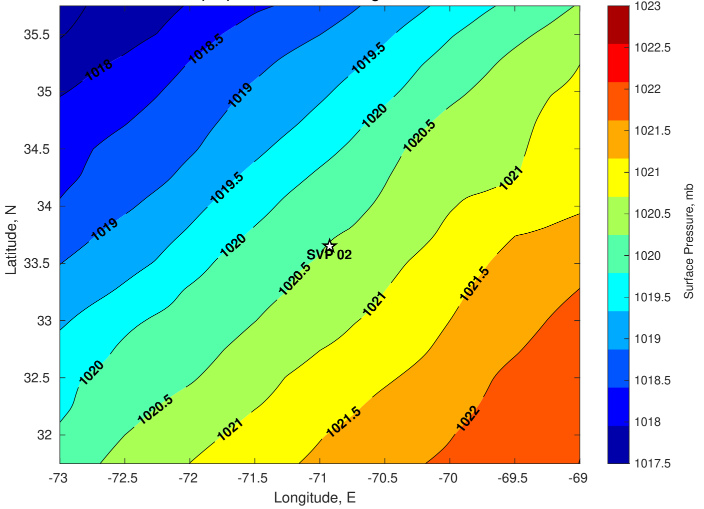
Surface Pressure (mb) for SVP 02 at 01-Aug-2024 00:00:00
