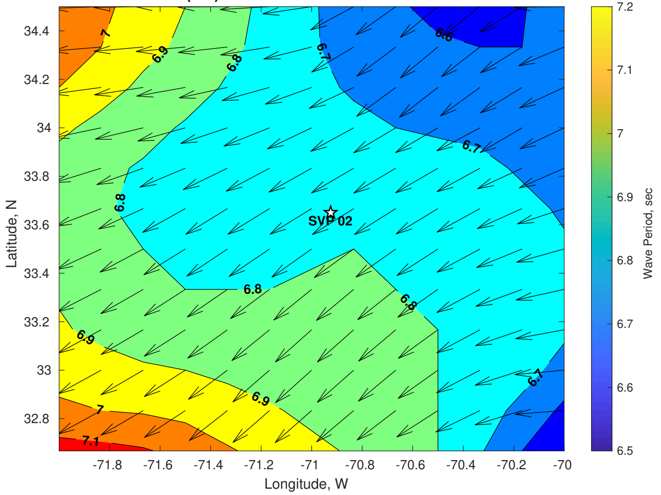
Wave Period (sec) for SVP 02 at 30-Jul-2024 06:00:00
