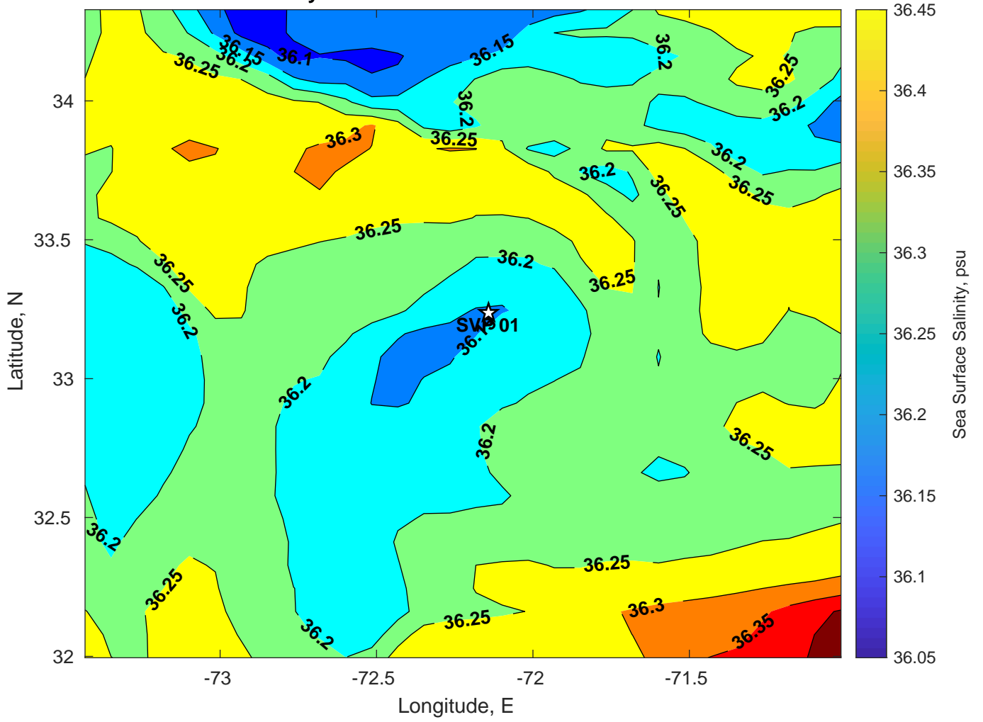
Surface Salinity for SVP 01 at 31-Jul-2024 00:00:00
