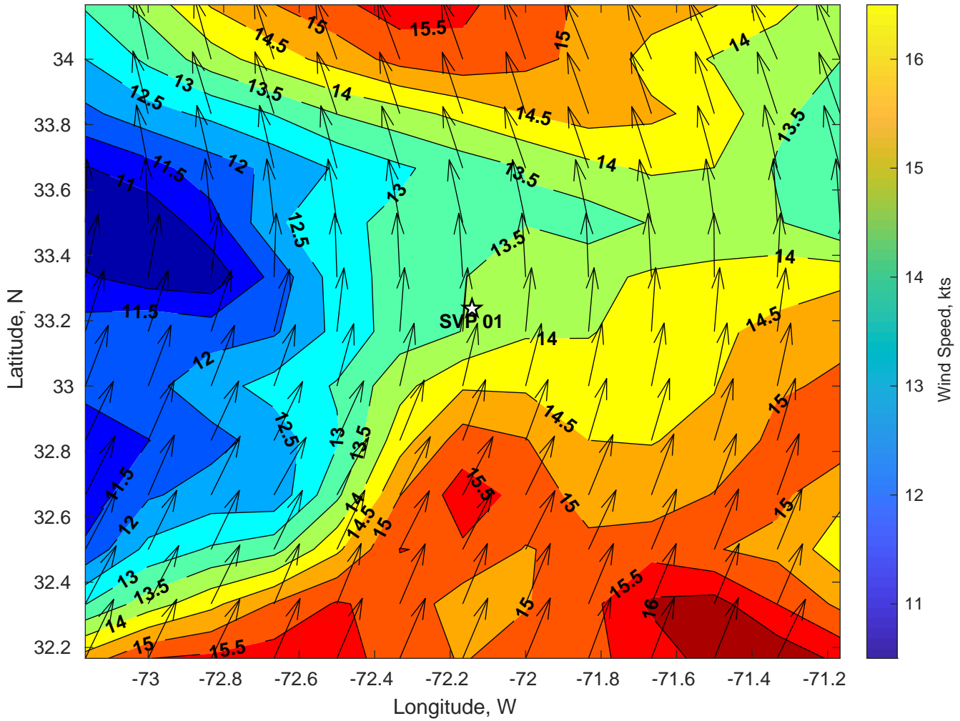
Winds (kts) for SVP 01 at 31-Jul-2024 06:00:00
