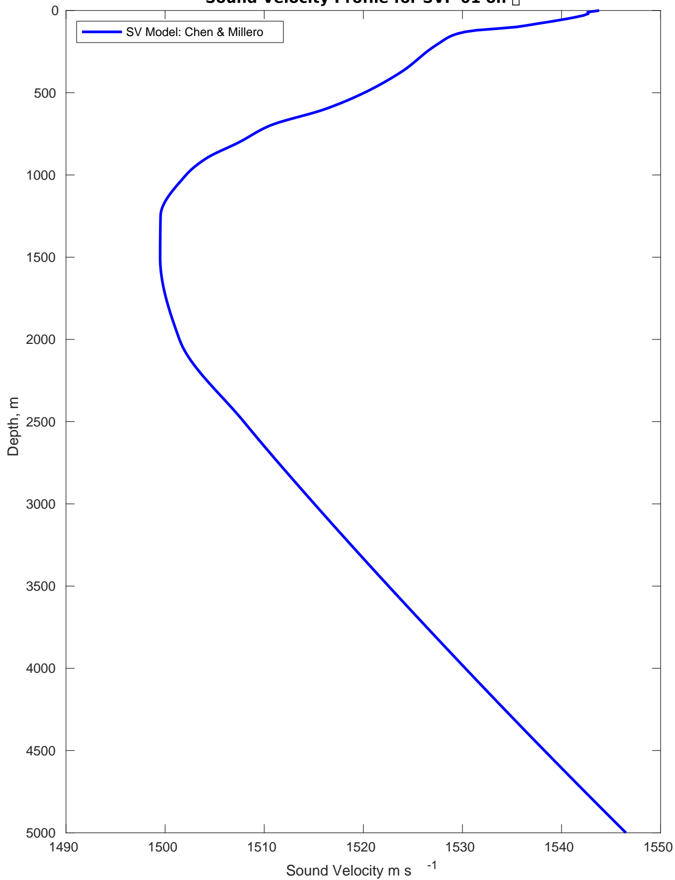
Sound Velocity Profile for SVP 01 on [ ]
