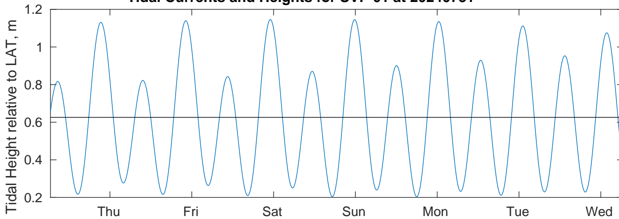
Tidal Currents and Heights for SVP 01 at 20240731
