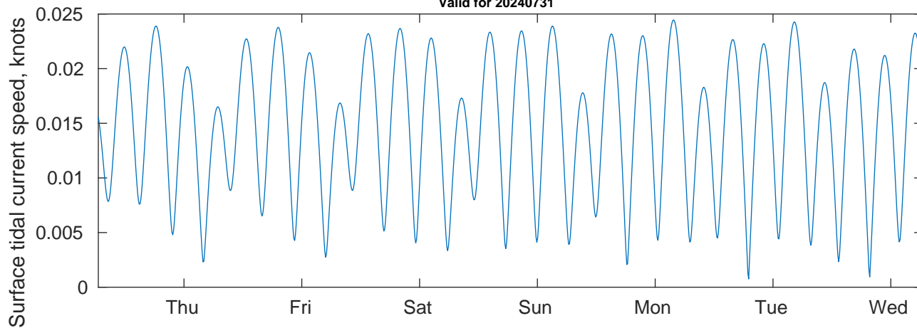
Tidal Currents and Heights for SVP 01 at 20240731
