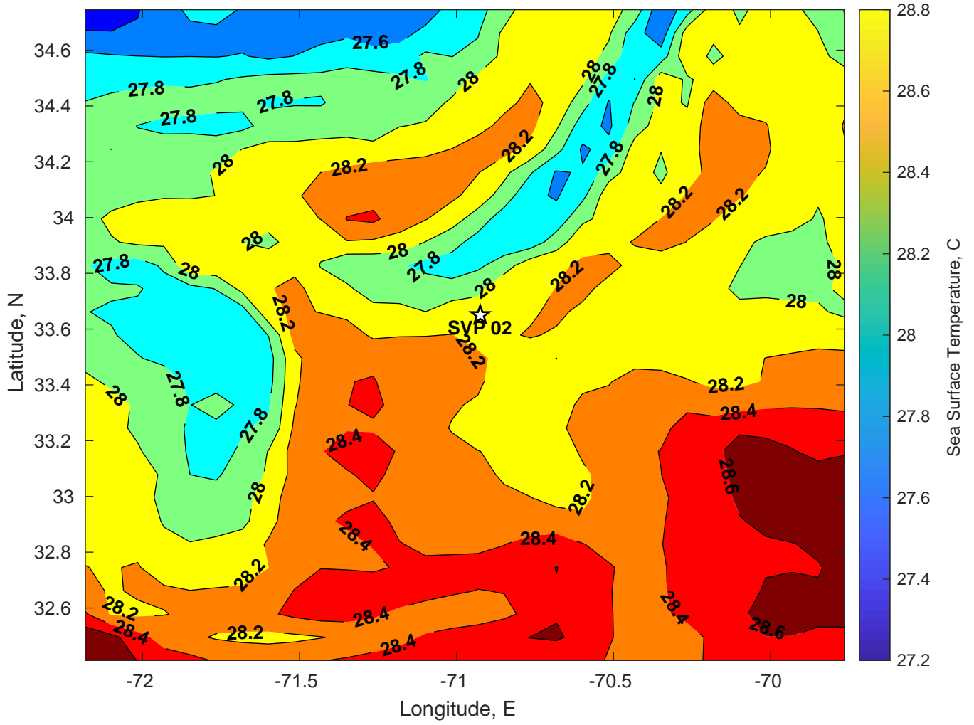
SST for SVP 02 at 31-Jul-2024 00:00:00
