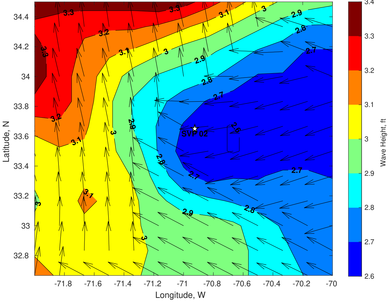
Wave Height (ft) for SVP 02 at 31-Jul-2024 06:00:00
