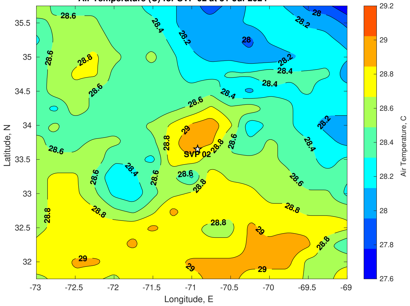
Air Temperature (C) for SVP 02 at 31-Jul-2024
