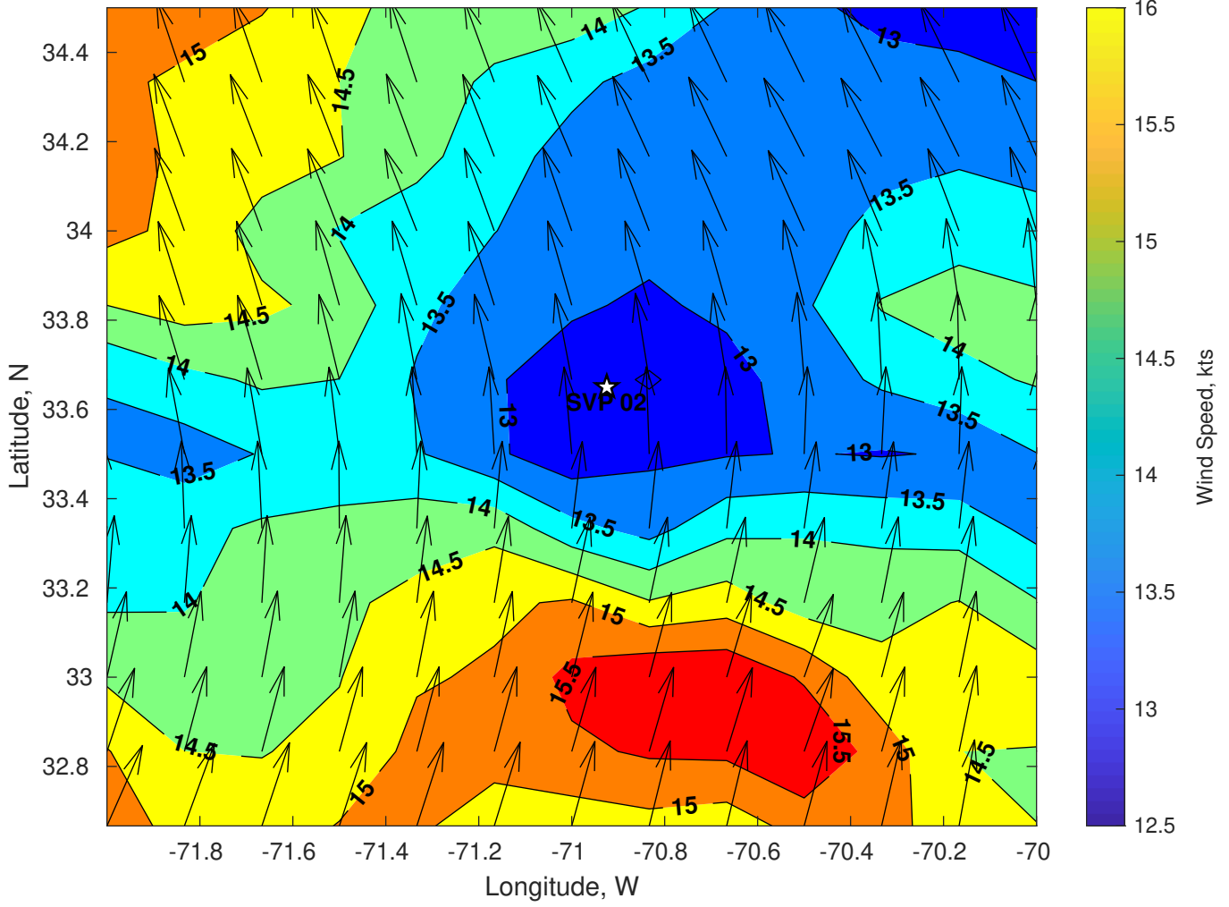
Winds (kts) for SVP 02 at 31-Jul-2024 06:00:00
