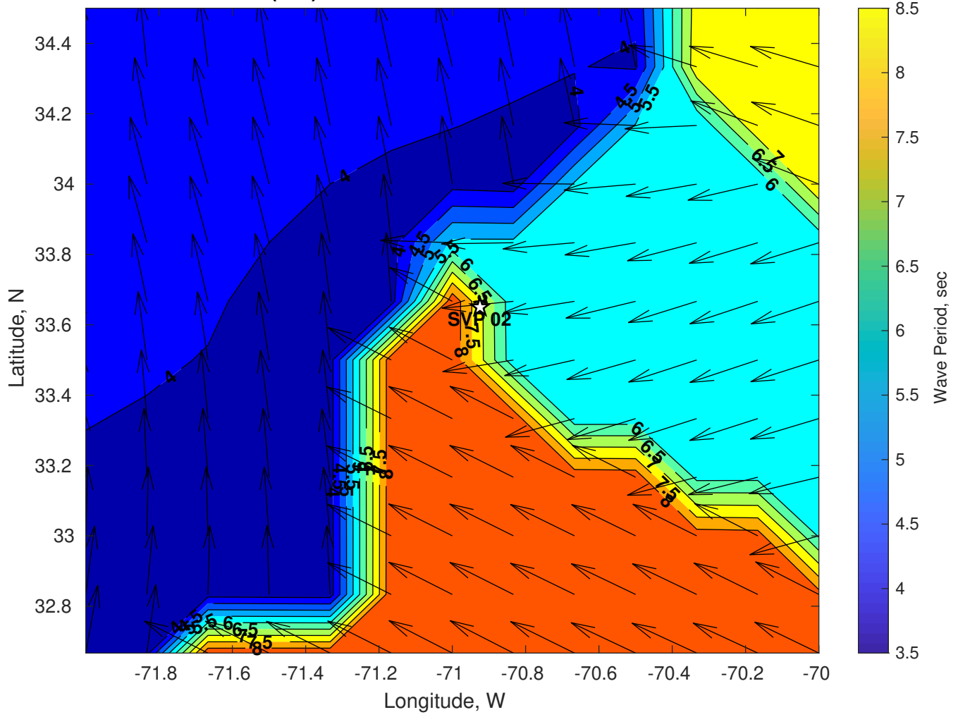
Wave Period (sec) for SVP 02 at 31-Jul-2024 06:00:00
