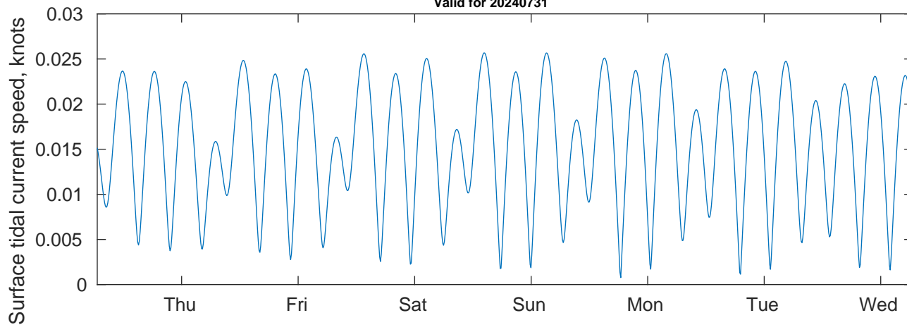
Tidal Currents and Heights for SVP 02 at 20240731
