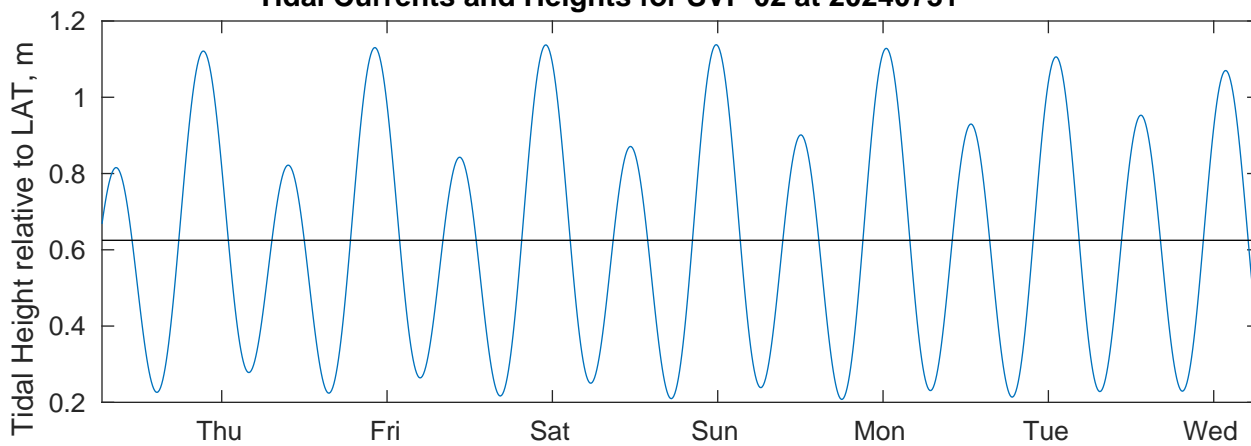
Tidal Currents and Heights for SVP 02 at 20240731
