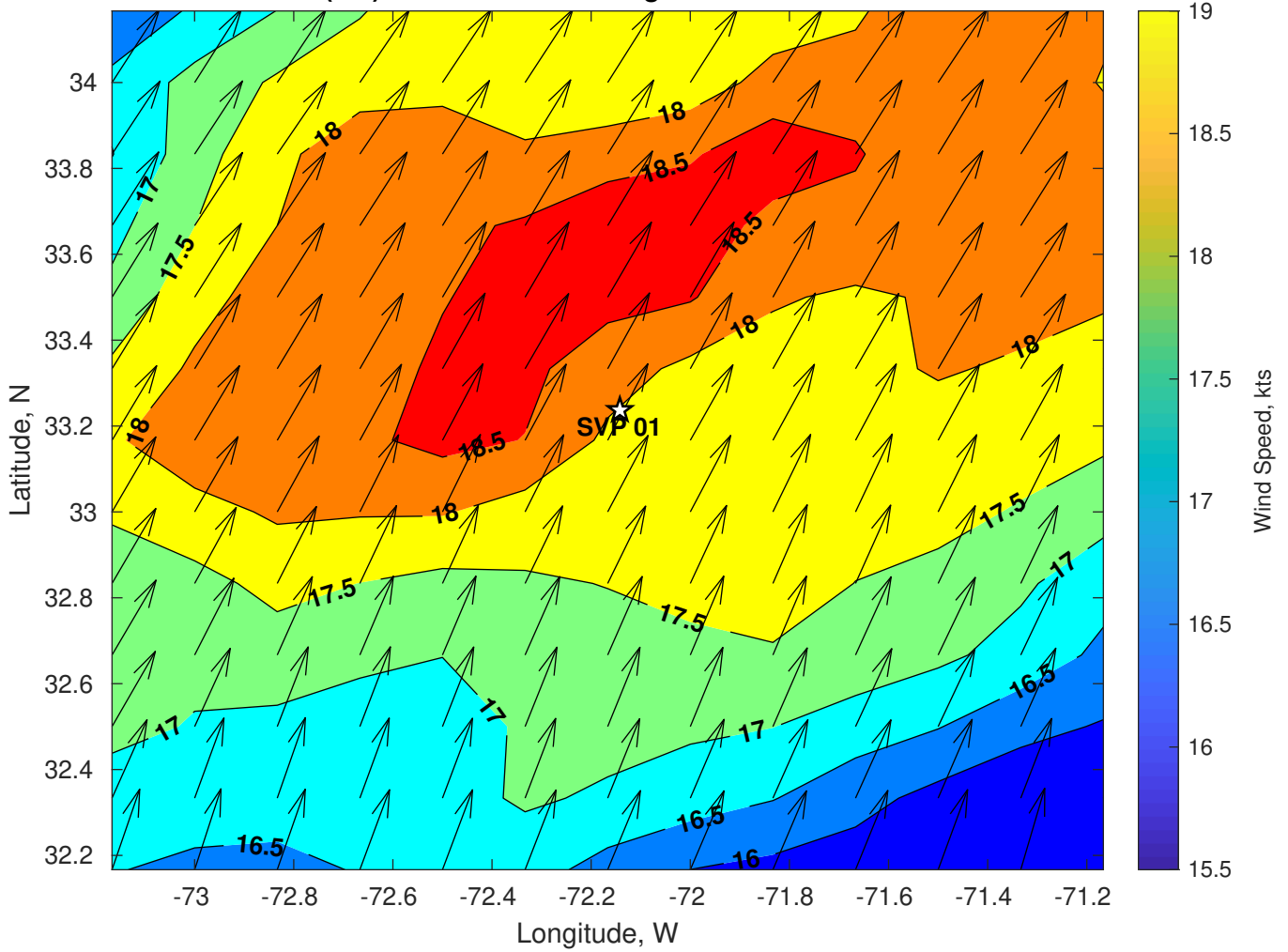
Winds (kts) for SVP 01 at 01-Aug-2024 06:00:00
