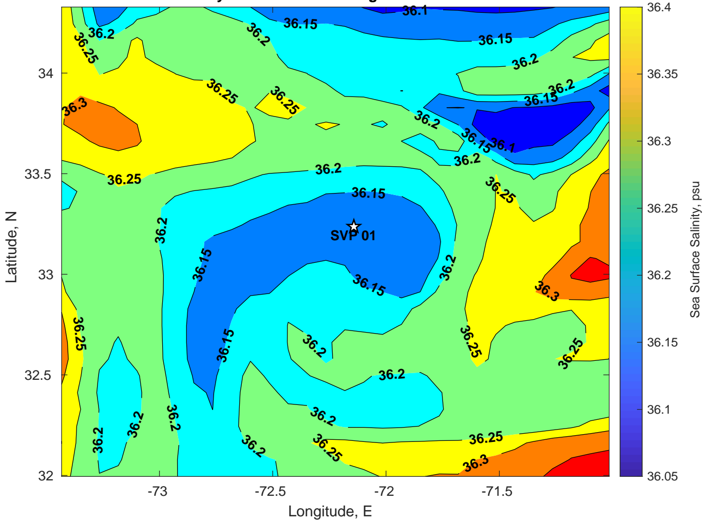
Surface Salinity for SVP 01 at 02-Aug-2024 00:00:00
