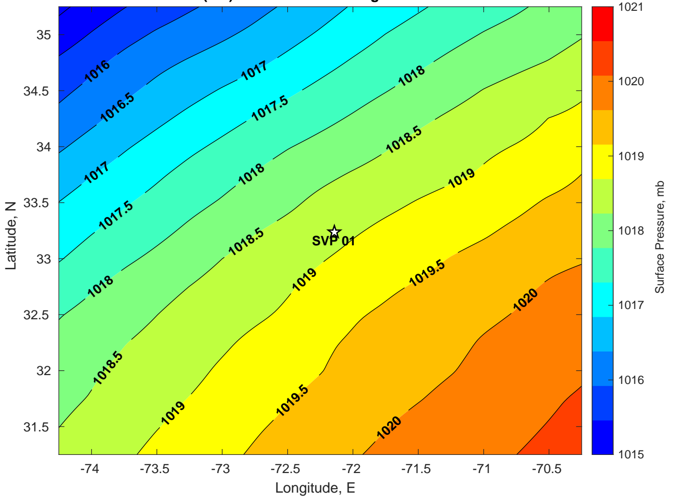
Surface Pressure (mb) for SVP 01 at 03-Aug-2024 00:00:00
