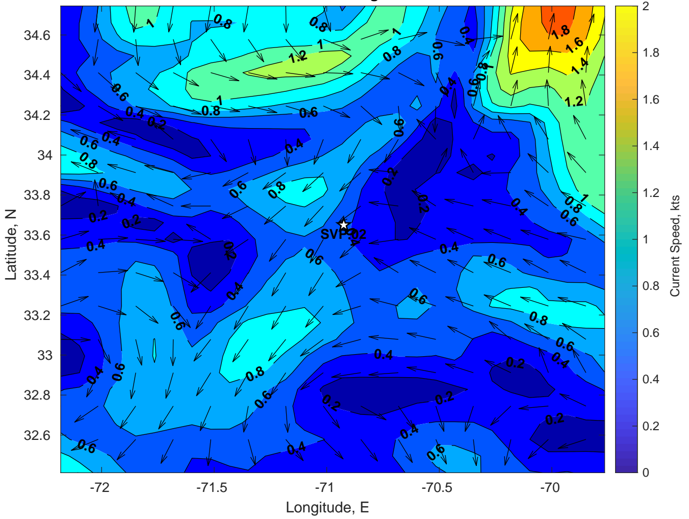
Surface Currents for SVP 02 at 01-Aug-2024 00:00:00
