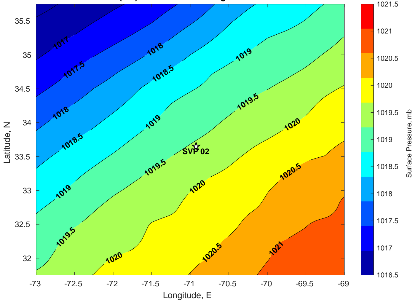
Surface Pressure (mb) for SVP 02 at 03-Aug-2024 00:00:00
