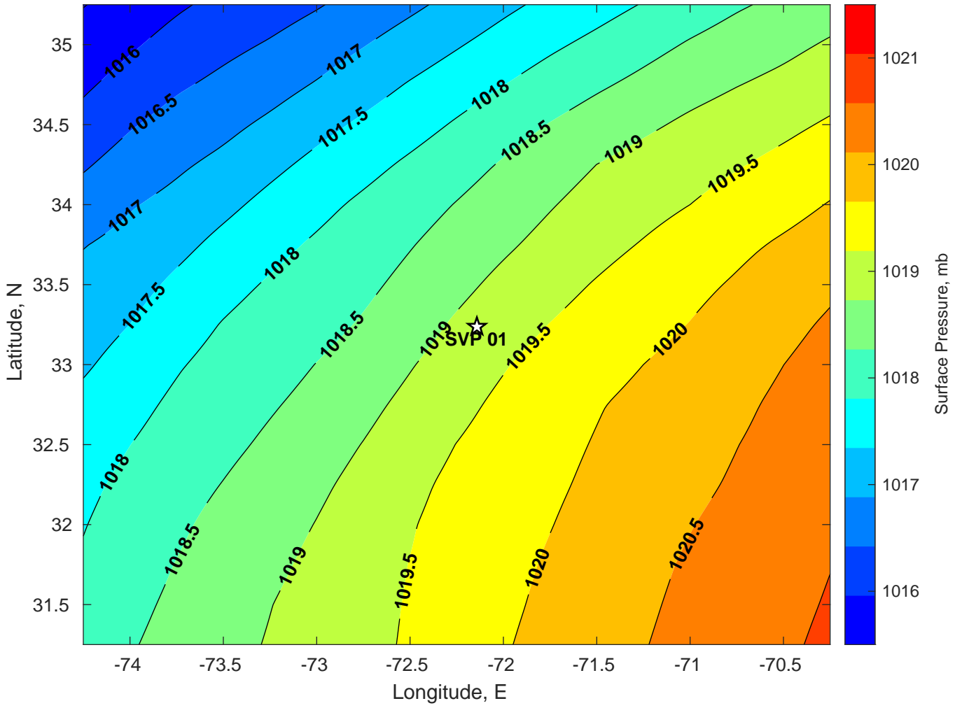
Surface Pressure (mb) for SVP 01 at 04-Aug-2024 00:00:00
