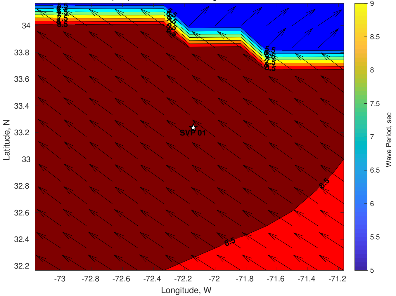
Wave Period (sec) for SVP 01 at 03-Aug-2024 06:00:00
