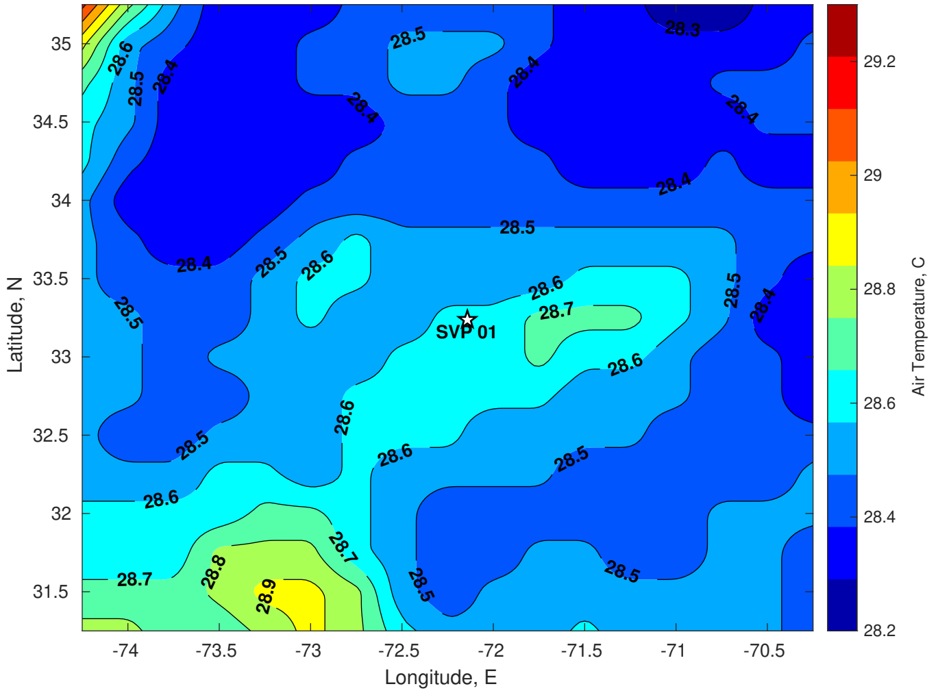
Air Temperature (C) for SVP 01 at 03-Aug-2024
