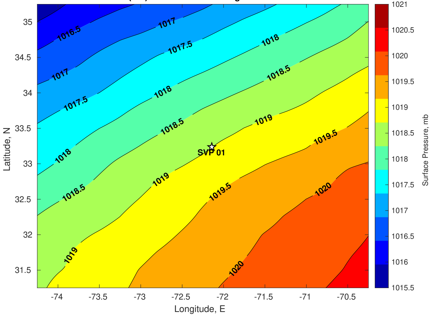
Surface Pressure (mb) for SVP 01 at 03-Aug-2024 00:00:00
