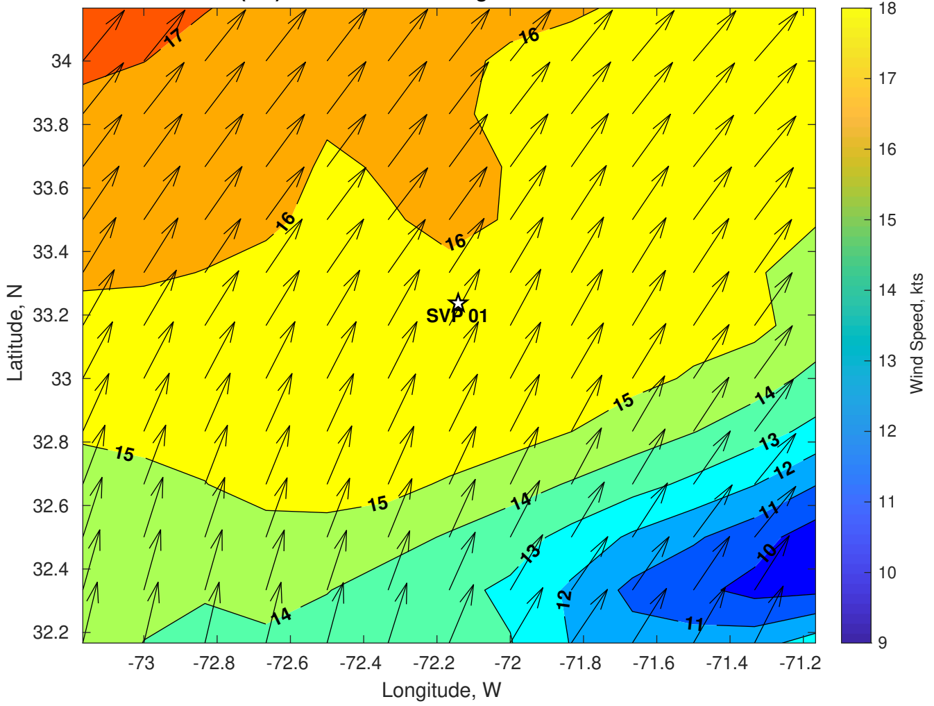
Winds (kts) for SVP 01 at 03-Aug-2024 06:00:00
