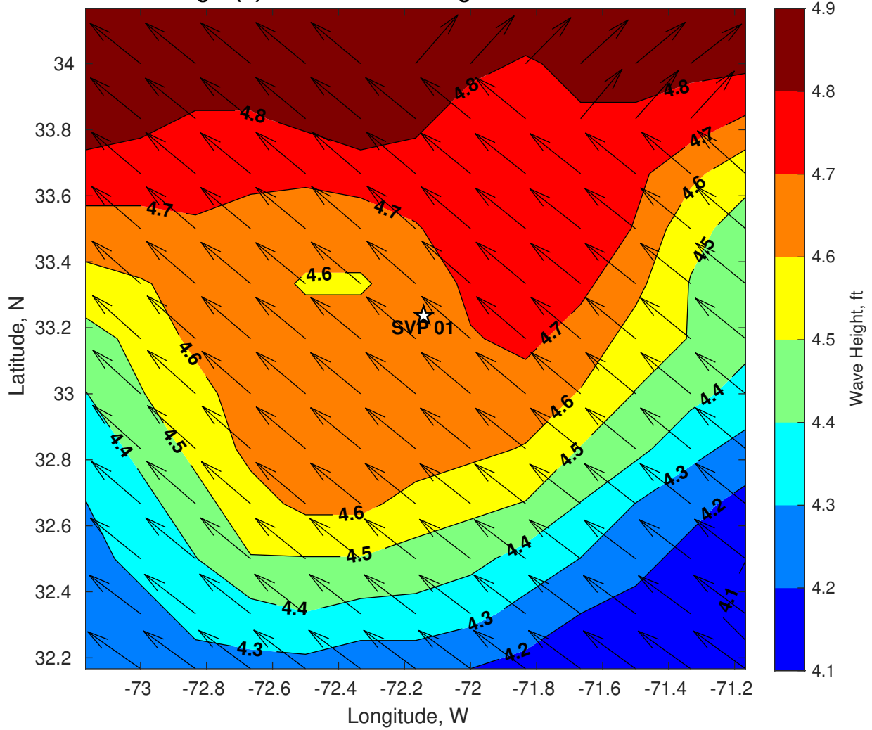
Wave Height (ft) for SVP 01 at 03-Aug-2024 06:00:00
