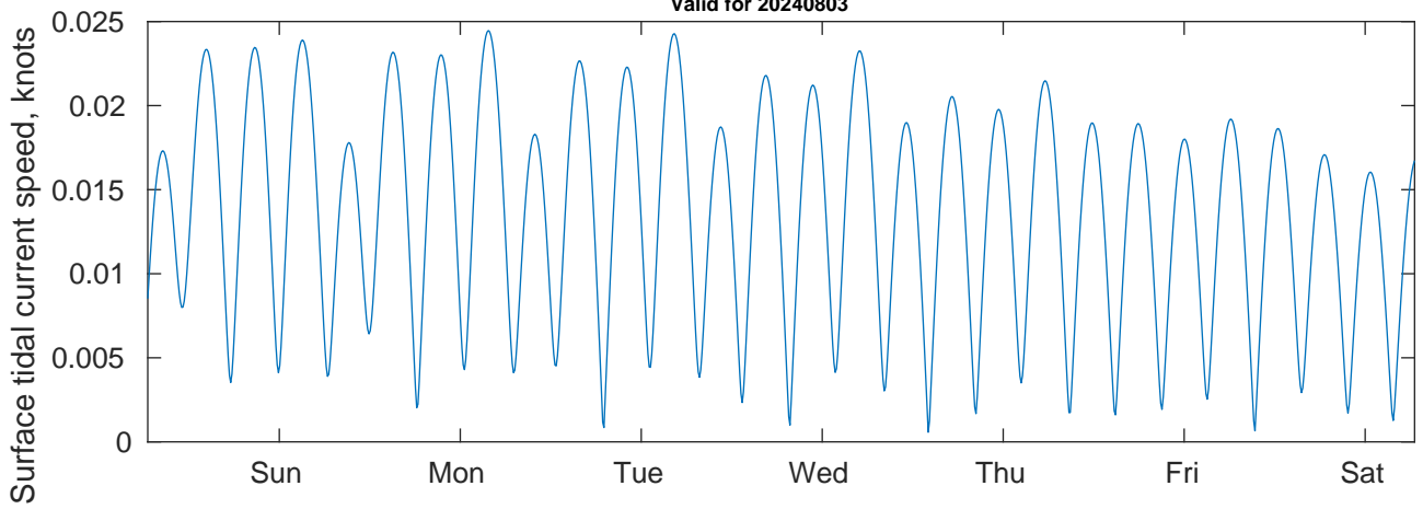
Tidal Currents and Heights for SVP 01 at 20240803
