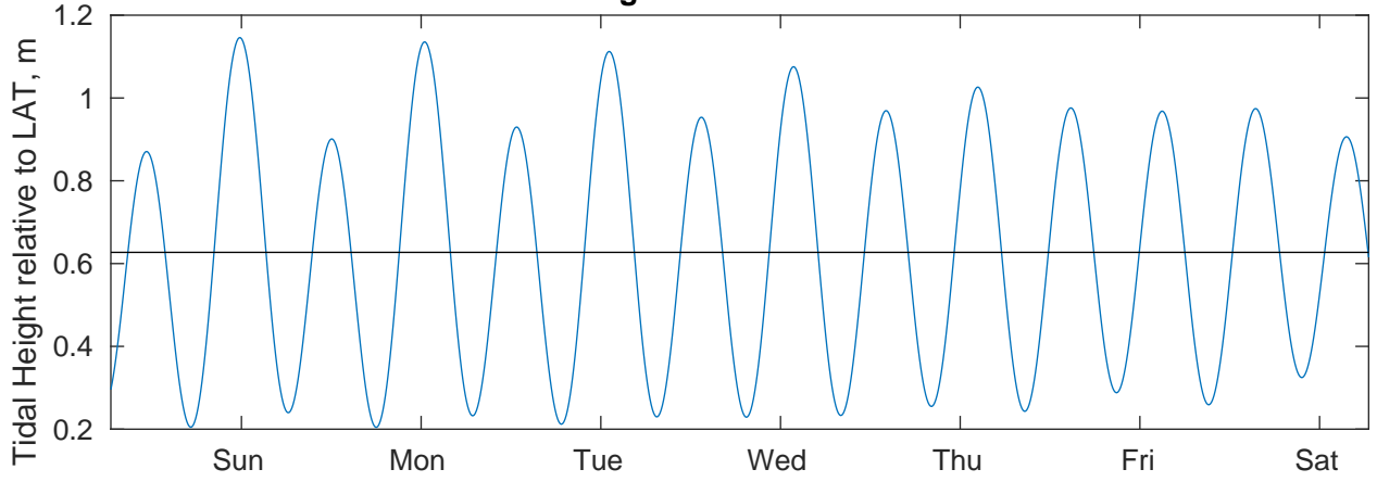
Tidal Currents and Heights for SVP 01 at 20240803
